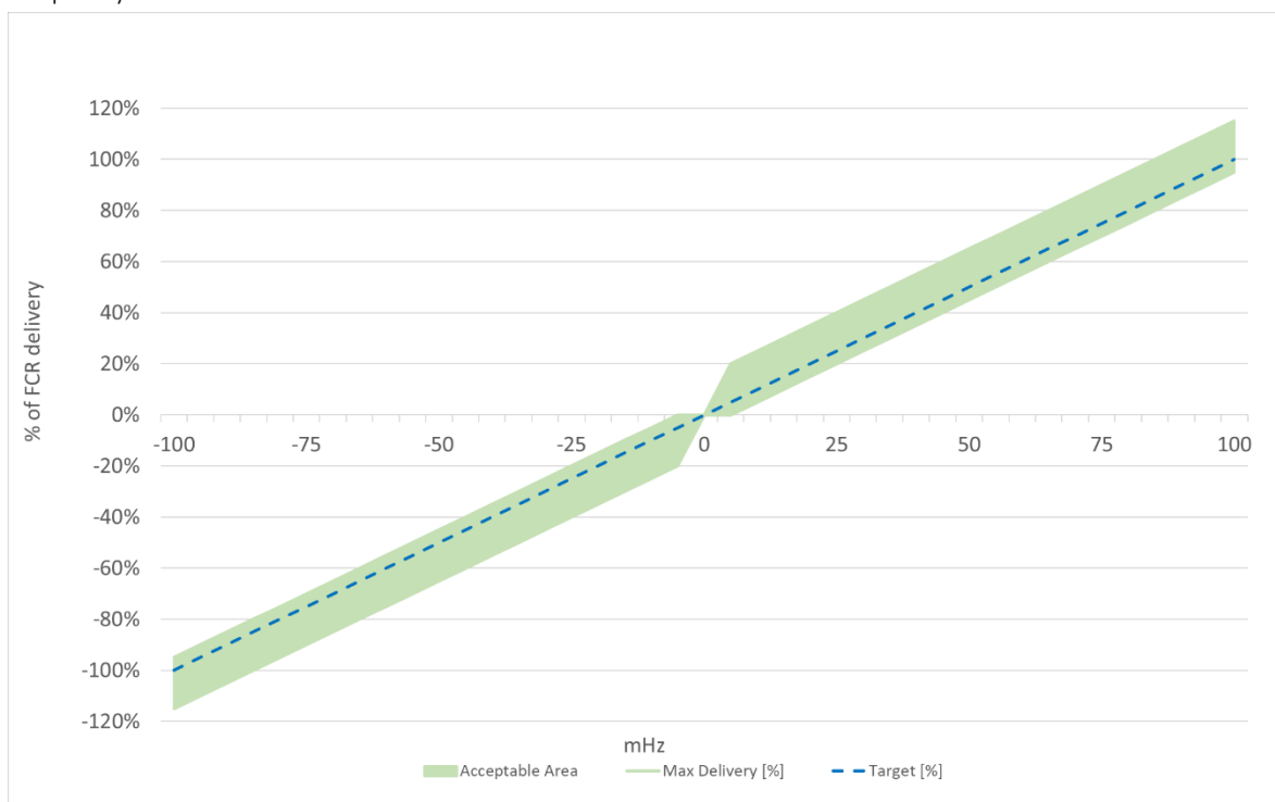
Figure 18 - Activation frequencies for FCR-N ranging with \pm 100 mHz from 50 Hz.
