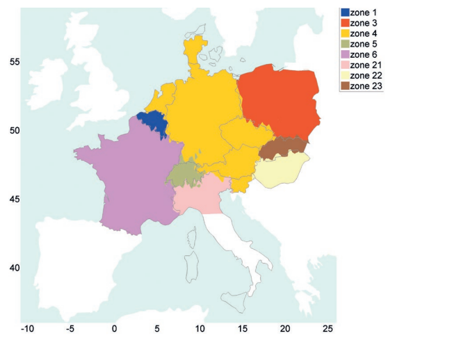
Figure 4.21: Clustering outcome, post adjustment steps 1–4, demonstrating the limitations of the modelling, 2025 SOAF worst case grid (after post-processing steps 1–4)
