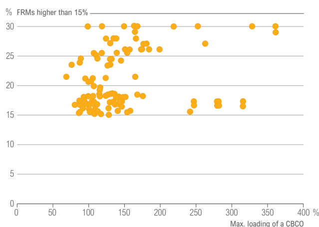
Impact of the loading of a CBCO on FRMs – Focus on high FRMs only
