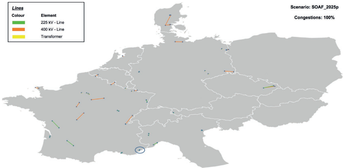
Figure 4.28: All N-0 grid constraints per voltage level in the SOAF 2025 planned scenario – based on the assumption of a full implementation of the planned network extensions
