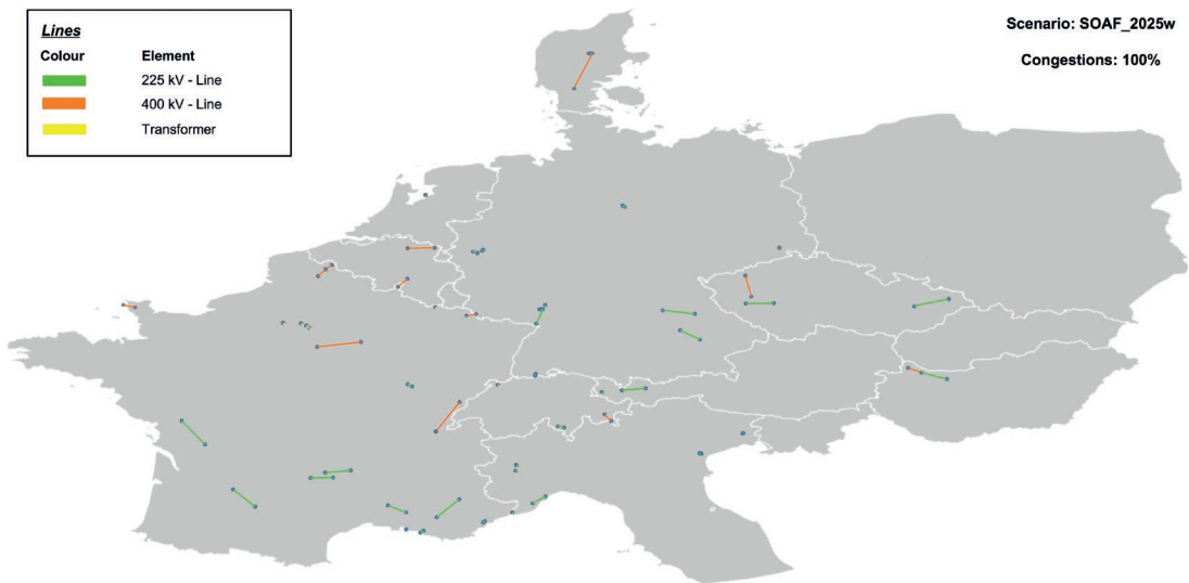
Figure 4.29: All N-0 grid constraints per voltage level in the SOAF 2025 worst case scenario – based on the assumption of an only partial implementation of the planned network extensions
