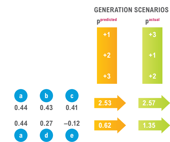
Figure 2.3: If nodes a, b and c inject 1, 2 and 3 units of power respectively, the power flow over the critical branch equals 2.53, whereas shifting the generation pattern to 3, 1, 2 leads to a slightly different result, i.e. 2.57 – the small difference of power flow is caused by the similarity of PTDF values in 'zone' a + b + c .
