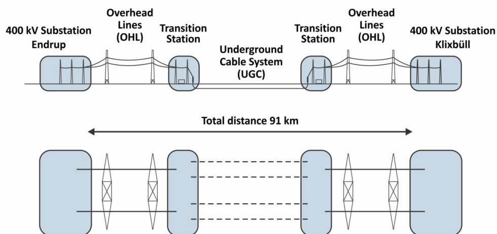
Figure 36 400 kV transmission line - Endrup-Klxbüll.
