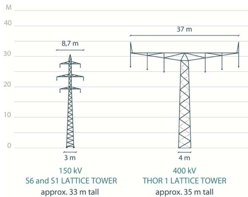
Figure 11: Left: Existing 150 kV OHL tower design between Endrup and Idomlund.
