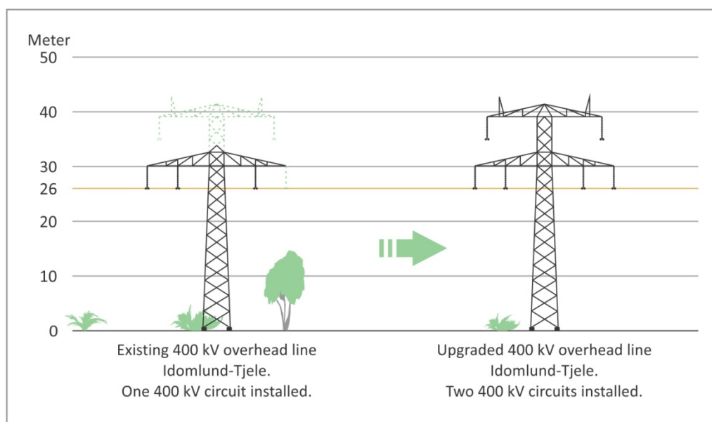
Figure 9 Proposed refitting of existing 400 kV Donau towers.
