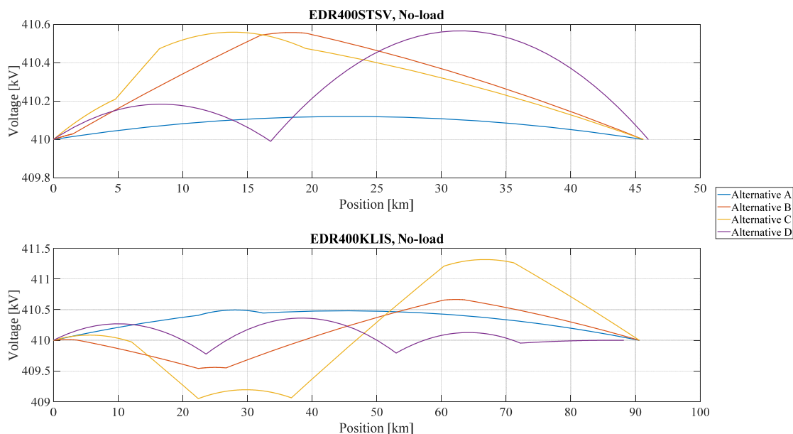
Figure 38: No-load voltage profiles of Endrup-Stovstrup and Endrup-Klxbüll at a fixed voltage of 410 kV at both end terminals. Approximately 100 % reactive compensation is applied.
