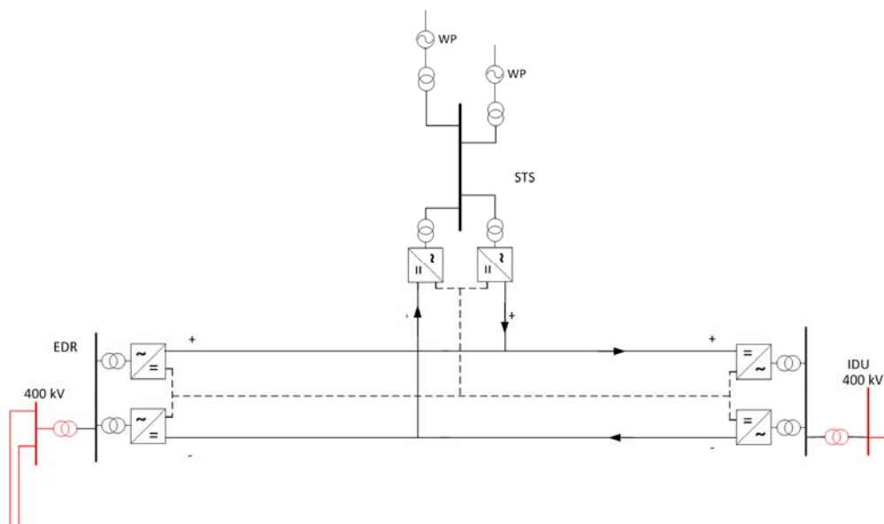
Figure 24: Two three-terminal HVDC links configured as bipoles exemplified using the Endrup-Idumlund transmission line.
