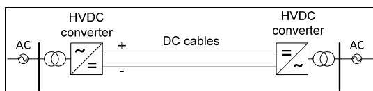
Figure 20: Symmetrical monopole.
