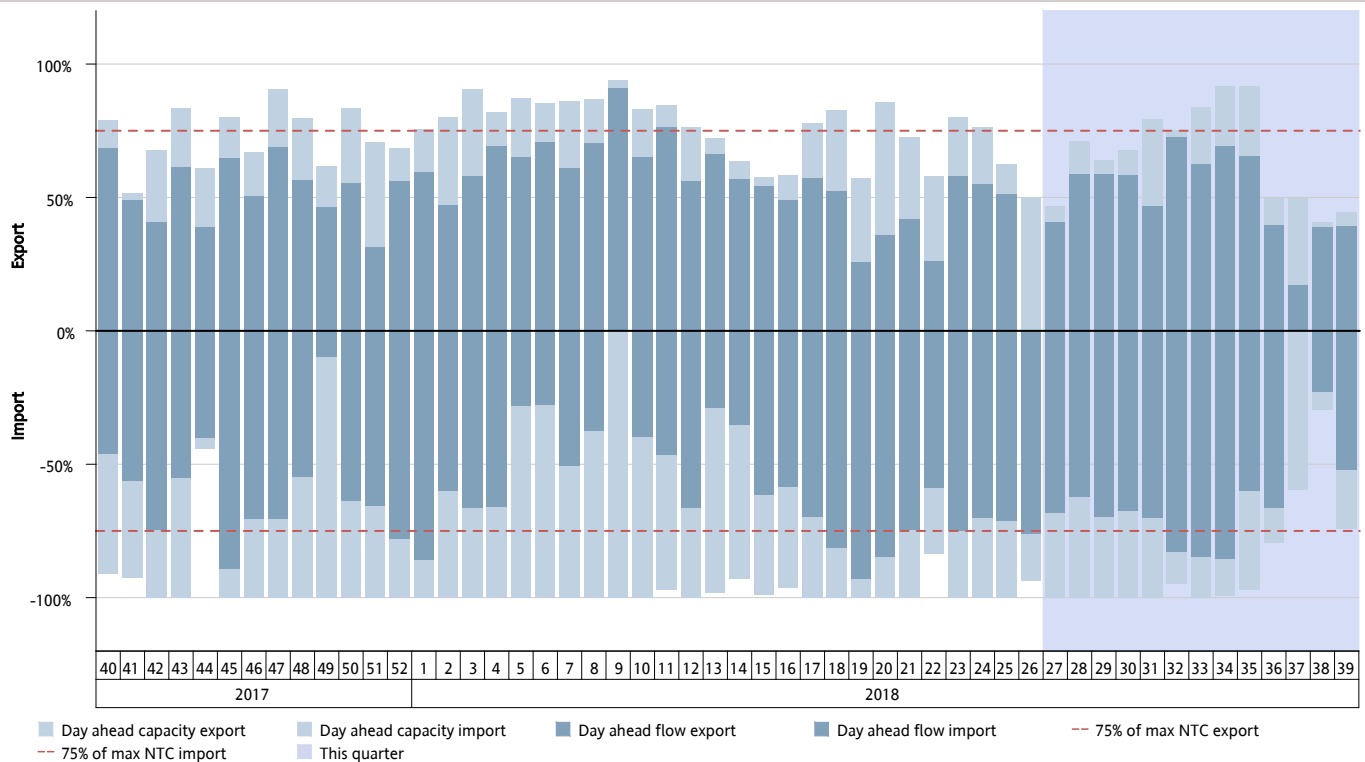
Figure 16: Shows cross-zonal day-ahead capacity result for the HVDC corridor DK1-SE3, showing average weekly capacity given and flow as a percentage of max NTC. Available capacity is given for all hours, but the average flow is only given for hours with flow in that direction. Export indicates flow from DK1 to SE3, while import indicates flow from SE3 to DK1.
