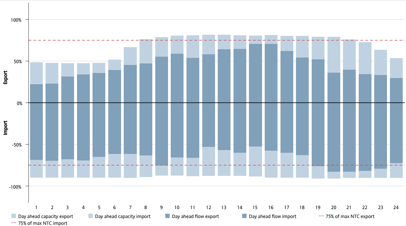
Figure 17: Shows cross-zonal day-ahead capacity result for the HVDC corridor DK1-SE3, showing average per hour of the day (1-24) capacity given and flow as a percentage of max NTC. Available capacity is given for all hours, but the average flow is only given for hours with flow in that direction. Export indicates flow from DK1 to SE3, while import indicates flow from SE3 to DK1.
