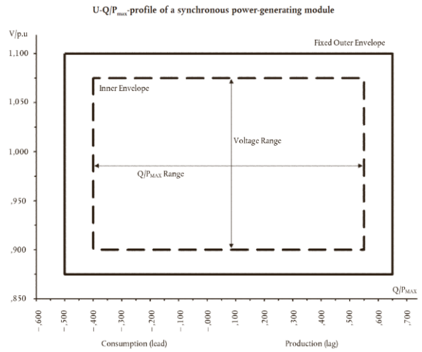
The diagram represents boundaries of a U-Q/P max -profile by the voltage at the connection point, expressed by the ratio of its actual value and the ref-
