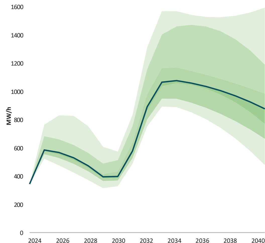
Figure 15 Median of projected need with 90 %,75 % and 10 % confidence intervals.
