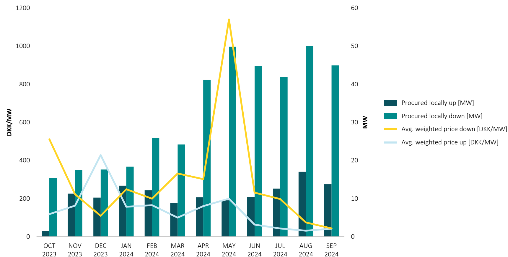
FIGURE 28 PROCURED FCR-D CAPACITY AND PRICES IN DK2 2023-2024
