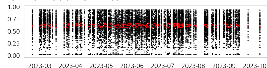
FIGURE 6 SIMULATED AND ACTUAL LOAD POINT DISTRIBUTION AT TOTAL LOAD POINT 0.6-0.7 FOR MEASURED DATA
