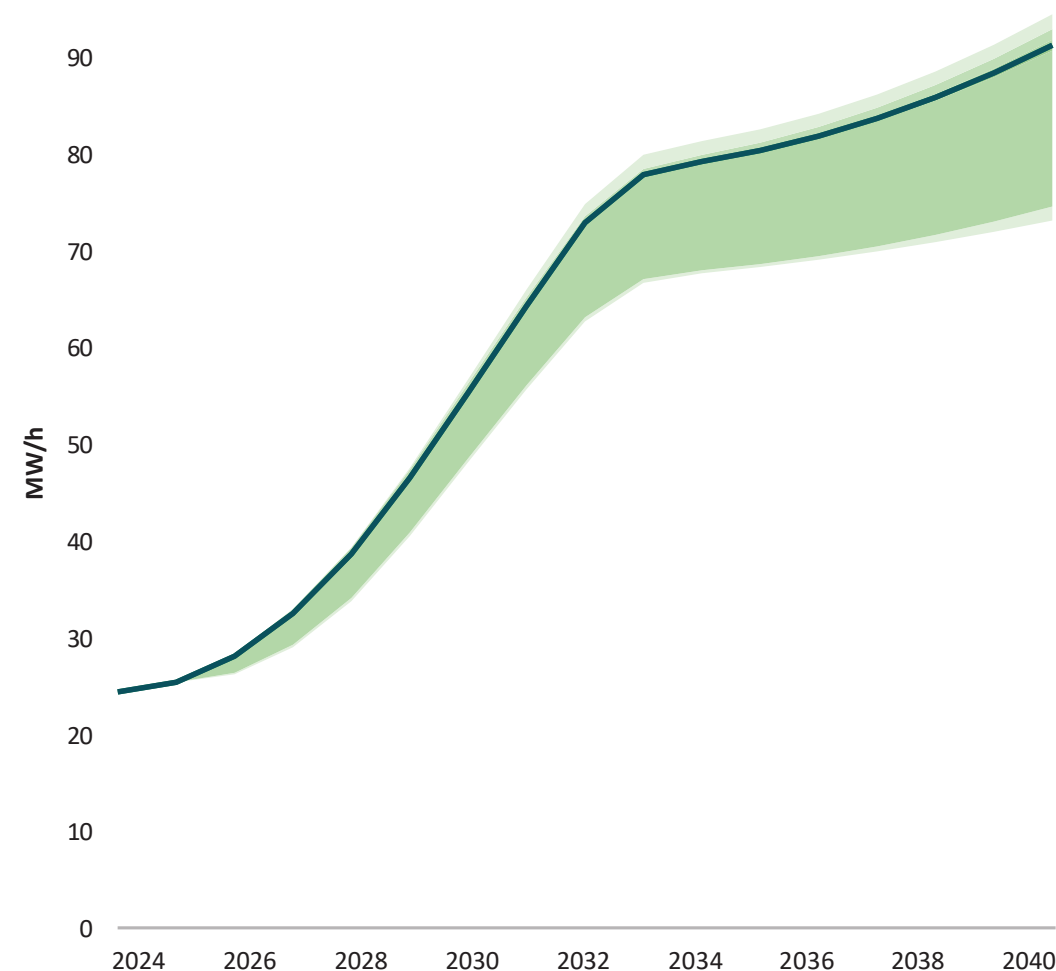
Figure 27 Median of projected need with 90 %,75 % and 10 % confidence intervals.
