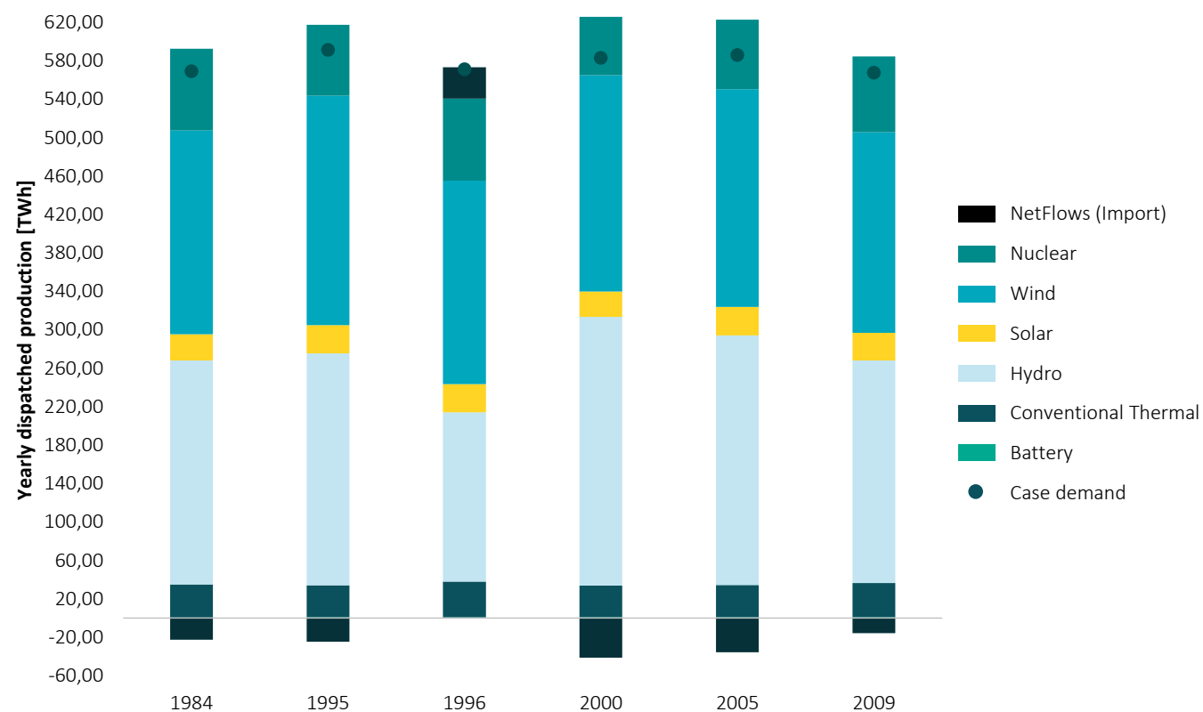
FIGURE 3 YEARLY DISPATCHED PRODUCTION IN THE NORDICS FOR SIMULATION YEAR 2030
