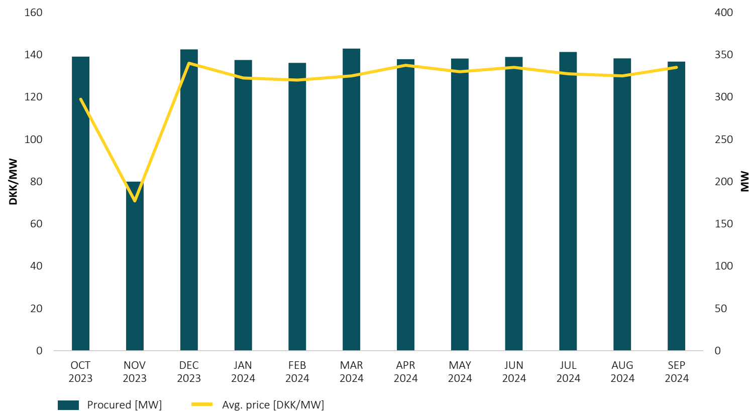
FIGURE 14 PROCURED mFRR CAPACITY AND PRICES IN THE MONTHLY AUCTION 2023-2024
