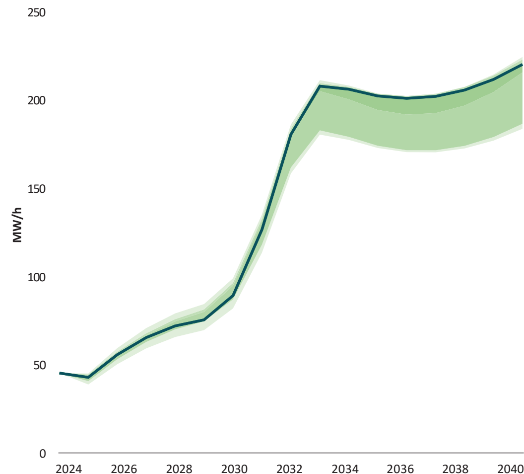
Figure 24 Median of projected need with 90 %,75 % and 10 % confidence intervals.
