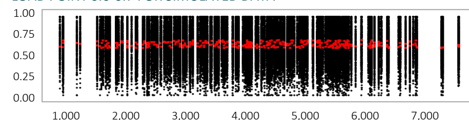
FIGURE 7 SIMULATED AND ACTUAL LOAD POINT DISTRIBUTION AT TOTAL LOAD POINT 0.6-0.7 FOR SIMULATED DATA
