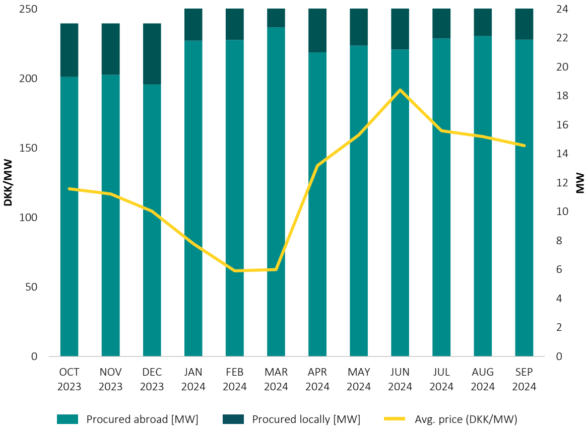
FIGURE 25 PROCURED FCR CAPACITY AND PRICES IN DK 1 2023-2024
