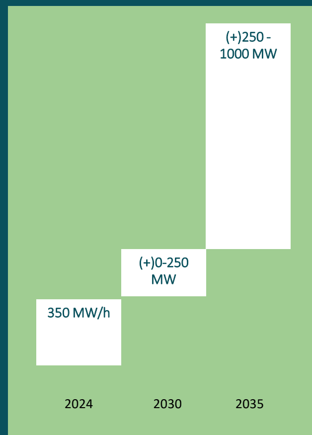
FIGURE 9 PROJECTED NEED FOR mFRR FOR UP-REGULATION IN DK1
