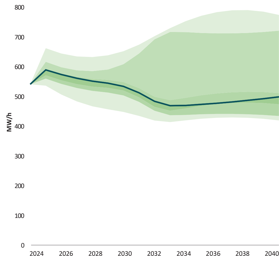
Figure 17 Median of projected need with 90 %,75 % and 10 % confidence intervals.
