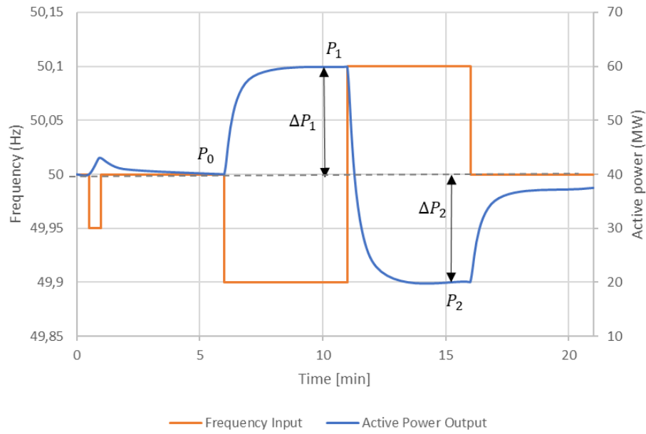
Figure 2. FCR-N step-response sequence. Input frequency (orange) and example response (blue).
