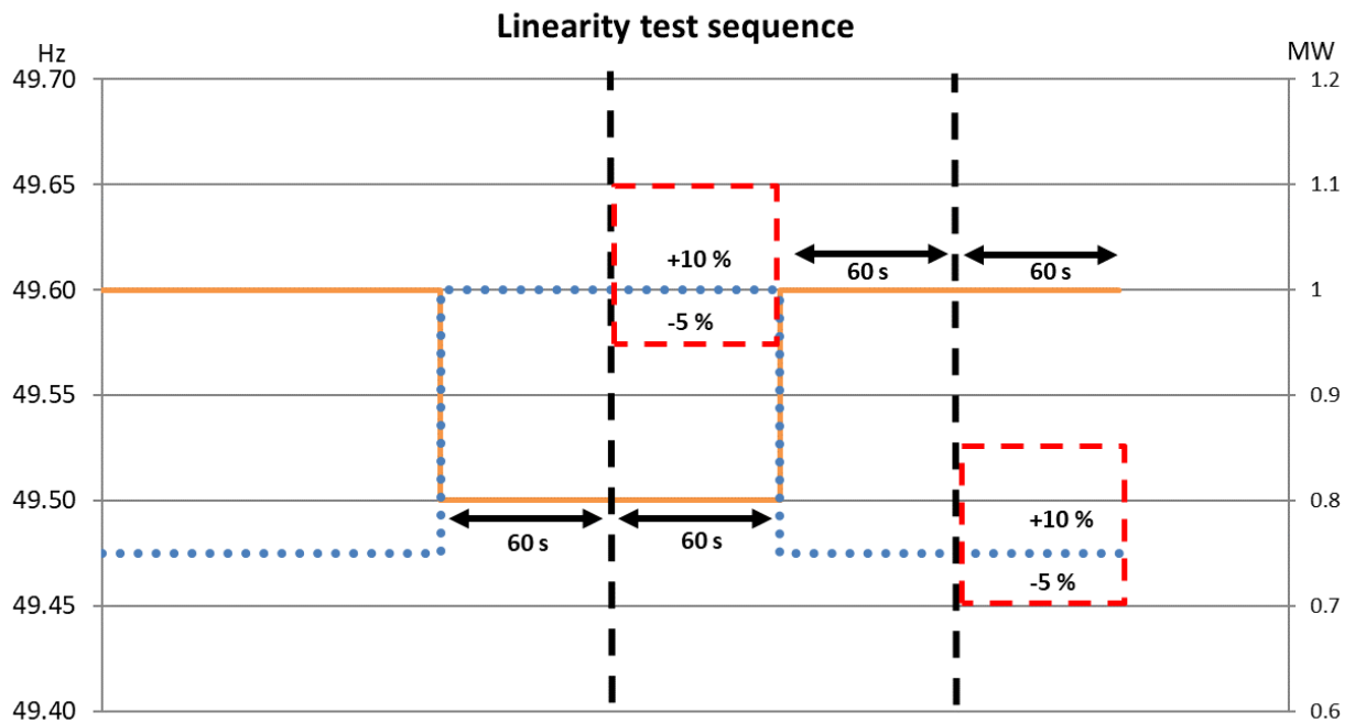
Figure 17. Allowed response area for FCR-D for the frequency steps from 49.6 Hz → 49.5 Hz → 49.6 Hz. The orange line is the frequency step. The blue dotted line is the directly proportional FCR response per MW. The red dashed squares indicate the allowed response area.
