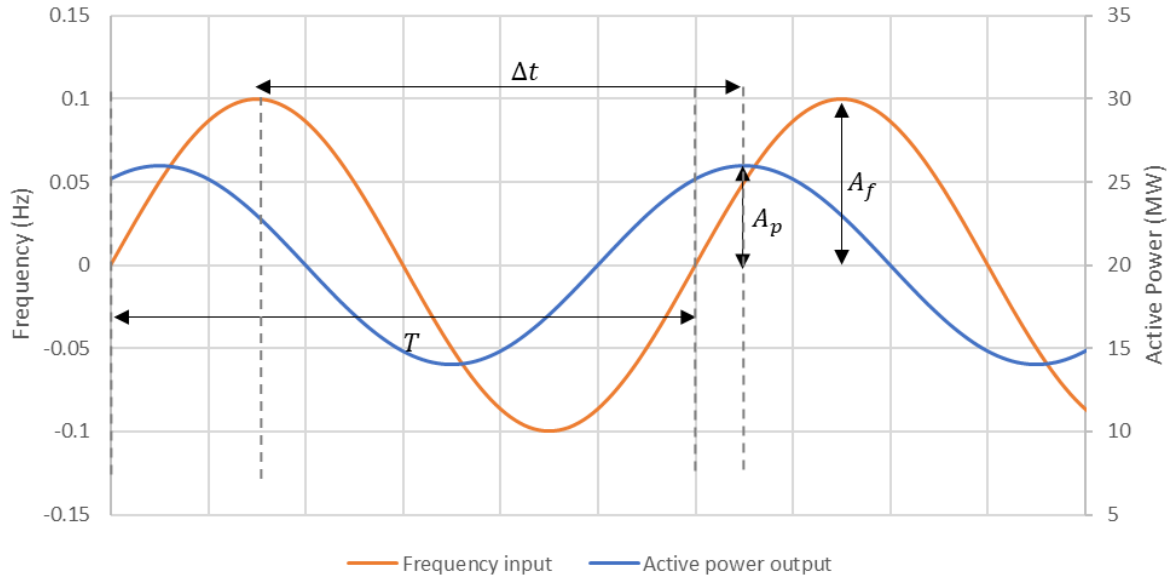
Figure 7. Example response (blue) from input frequency (orange) for FCR sine test.
