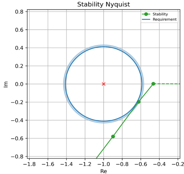
Figure 8. Illustration of the Nyquist stability criterion. The green dots correspond to the open loop system response calculated from each of the sine tests, the green line is an interpolation between those points. To fulfil the stability requirement, the green curve must pass outside and to the right of the light blue circle with radius r = 0.43 drawn around the point (-1,0j) , which is marked by a red cross. Results that are just slightly inside the light blue circle but still outside the dark blue circle will be accepted.
