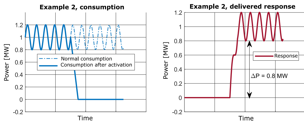
Figure 22. Example response where the variations are not independent of the delivered response.
