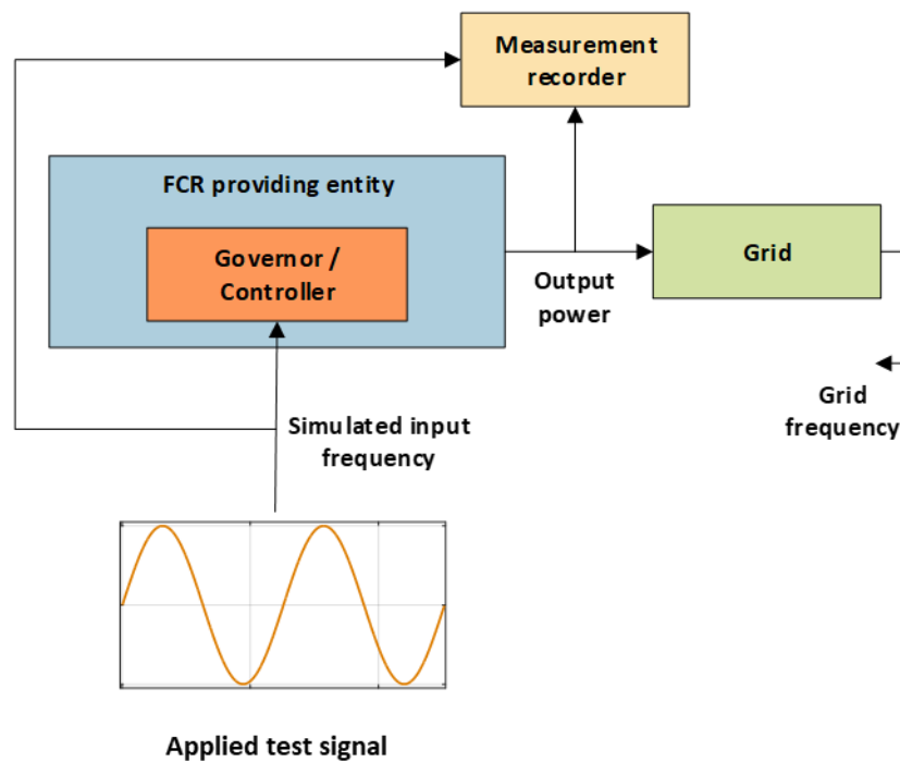
Figure 25. Test setup.
