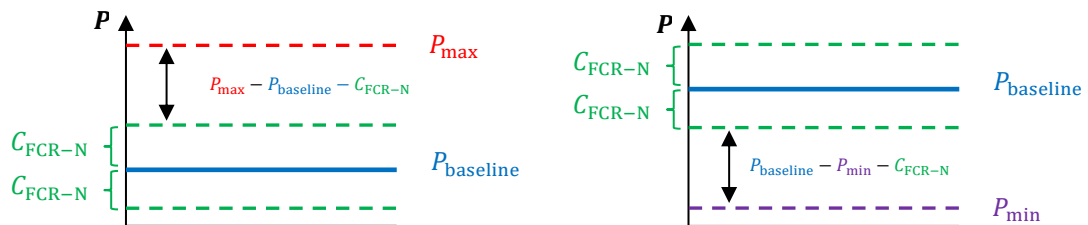
Figure 20. The limits of FCR-D capacity for an entity which is limited either by maximum active power or minimum active power while delivering FCR-N (FCR-D upwards in the left figure and FCR-D downwards in the right).
