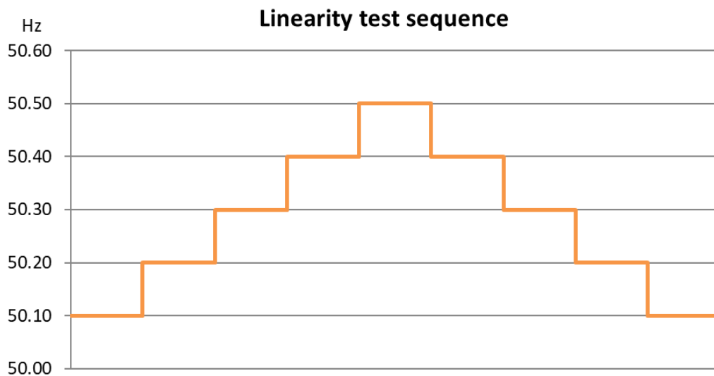
Figure 16: Grid frequency test signal for the FCR-D downwards linearity test.
