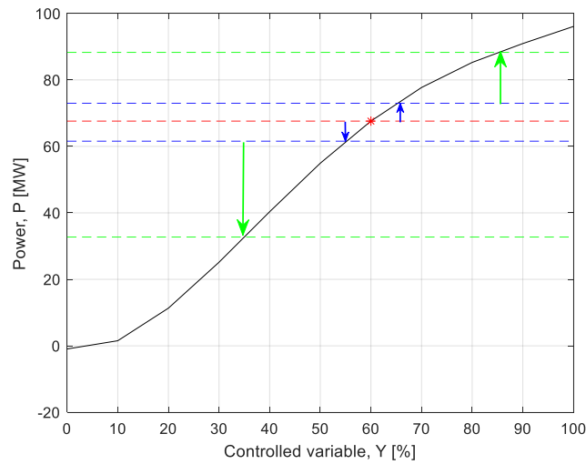
Figure 28. Illustration of the steady state power response of FCR-N and FCR-D. The black line is the steady state relation between the controlled variable Y and the power, the red star is the operating point, the blue lines show the power output at fully activated FCR-N and the green lines show the power output at fully activated FCR-D.
