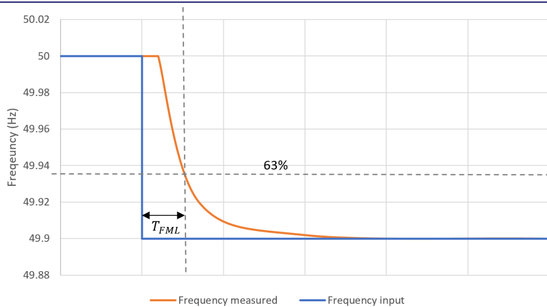
Figure 24. Example response (orange) from a separate test of frequency measurement loop, by applying a step frequency change (blue)
