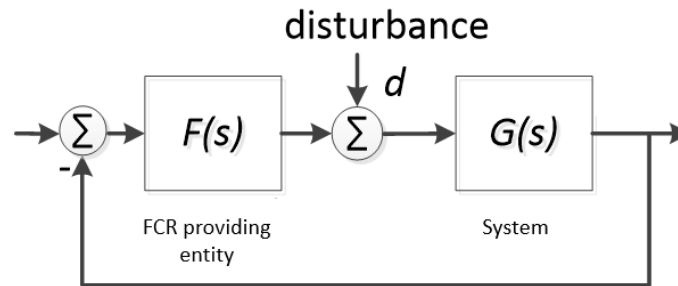
Figure 6. Illustration of the system used for evaluation of compliance with requirements in frequency domain.
