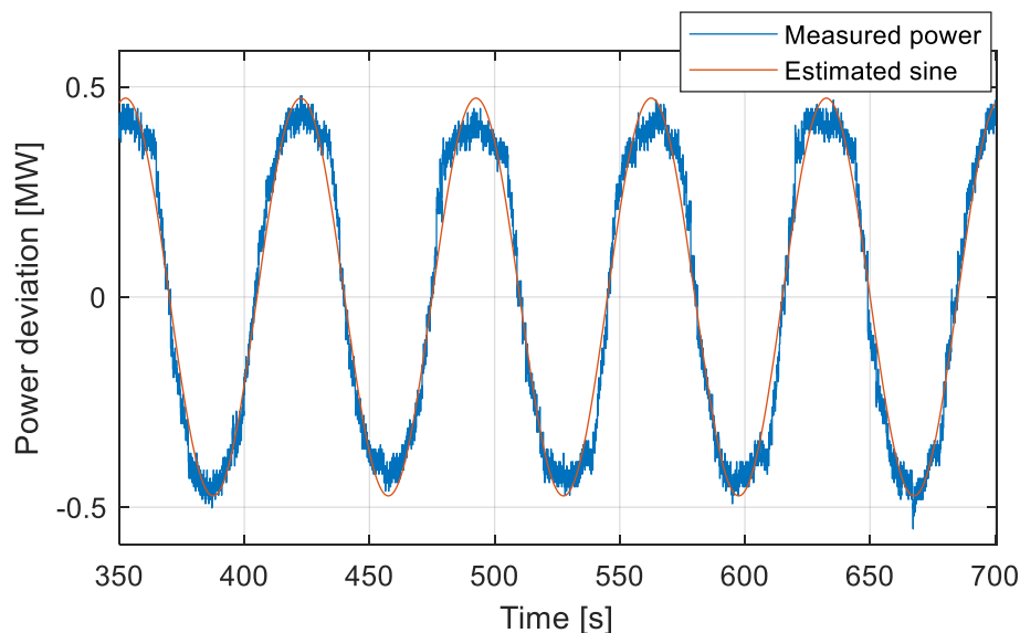
Figure 10. Example of the measured power from a sine test and the fitted sine.
