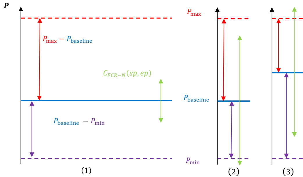
Figure 19. The three limits of FCR-N capacity for an entity which is limited either by prequalification test result (1), minimum active power (2) or maximum active power (3).
