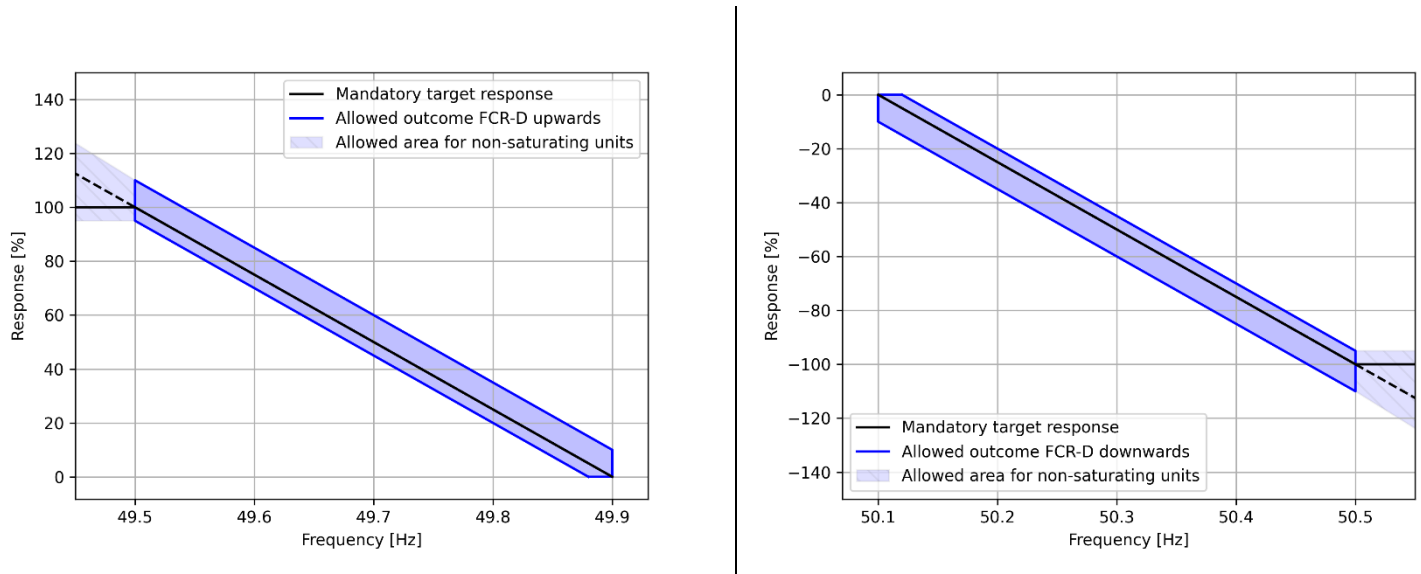
Figure 14. Activation of piecewise linear FCR-D resources. The black line indicates the mandatory target response. The controller shall be designed to minimise the deviation from the target response. The blue area defines the allowed outcome of the deviations, due to e.g. non-linear effects or step sizes for relay connected loads. The coordinates of the corners are provided in Table 8 below
