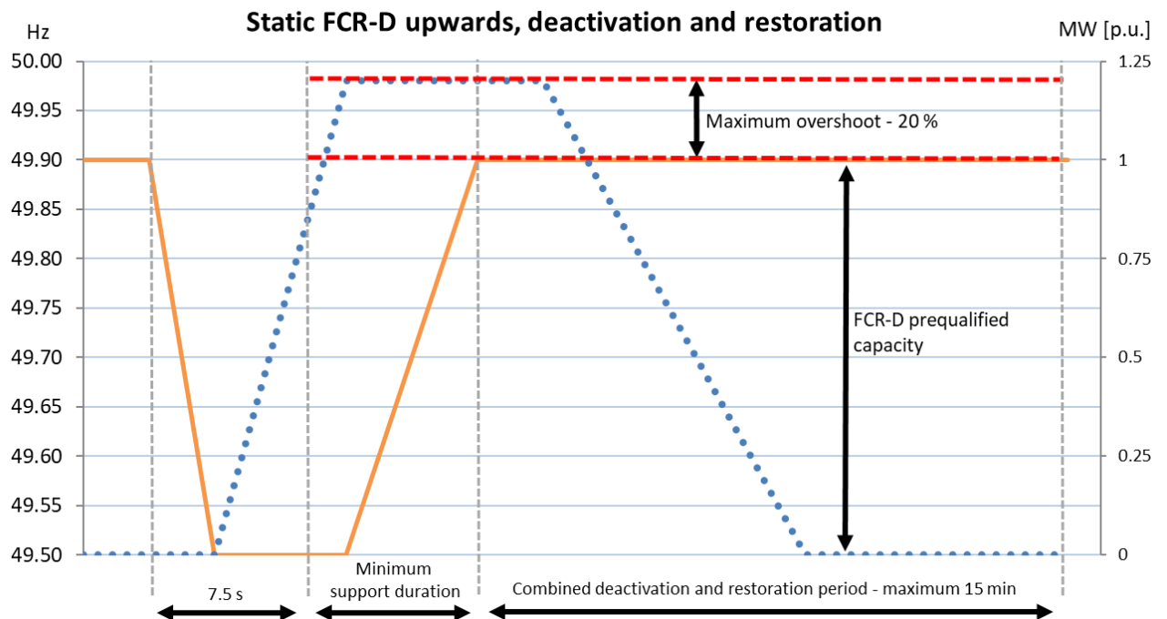
Figure 5. Maximum allowed overshoot and range for deactivation and restoration for static FCR-D. The orange line is an arbitrarily frequency ramp chosen to illustrate an allowed response from static FCR-D. The blue dotted line is an allowed response from static FCR-D.
