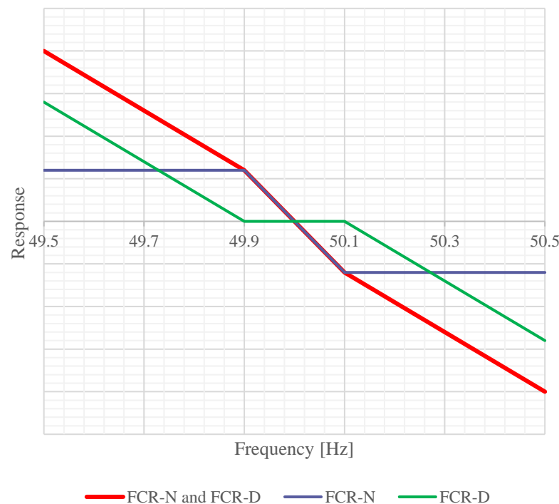
Figure 18. Steady state active power activation as a function of frequency, droop profile of FCR-N (blue), FCR-D (green) and both combined (red).
