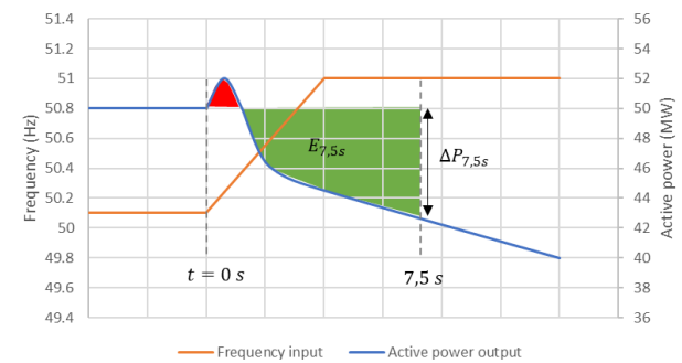
Figure 4. The left column shows the activation/deactivation requirements on ramp 1 and 2 for FCR-D upwards (top) and FCR-D downwards (bottom). The right column shows the dynamic performance requirements on ramp 5 for FCR-D upwards (top) and FCR-D downwards (bottom). The green area indicates positive energy contribution while the red area indicates negative energy contribution.
