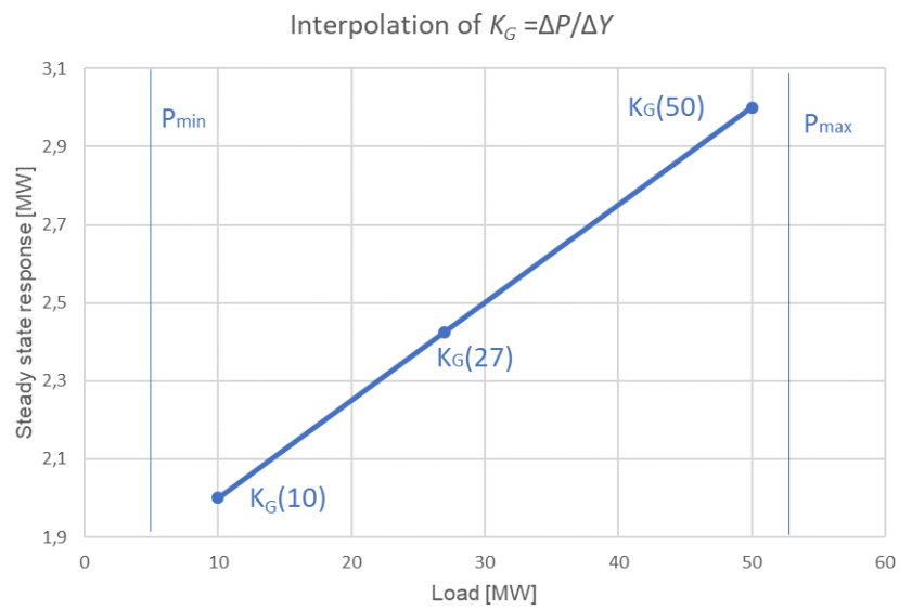
Figure 30. Example of interpolation of the load dependent gain K_G .
