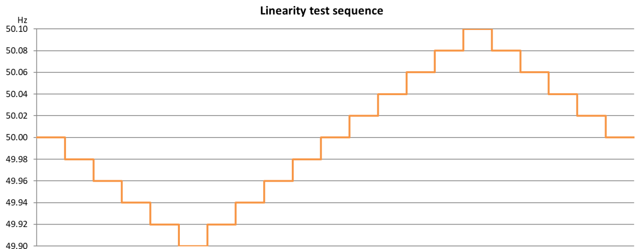
Figure 12. Grid frequency test signal for the FCR-N special linearity test.
