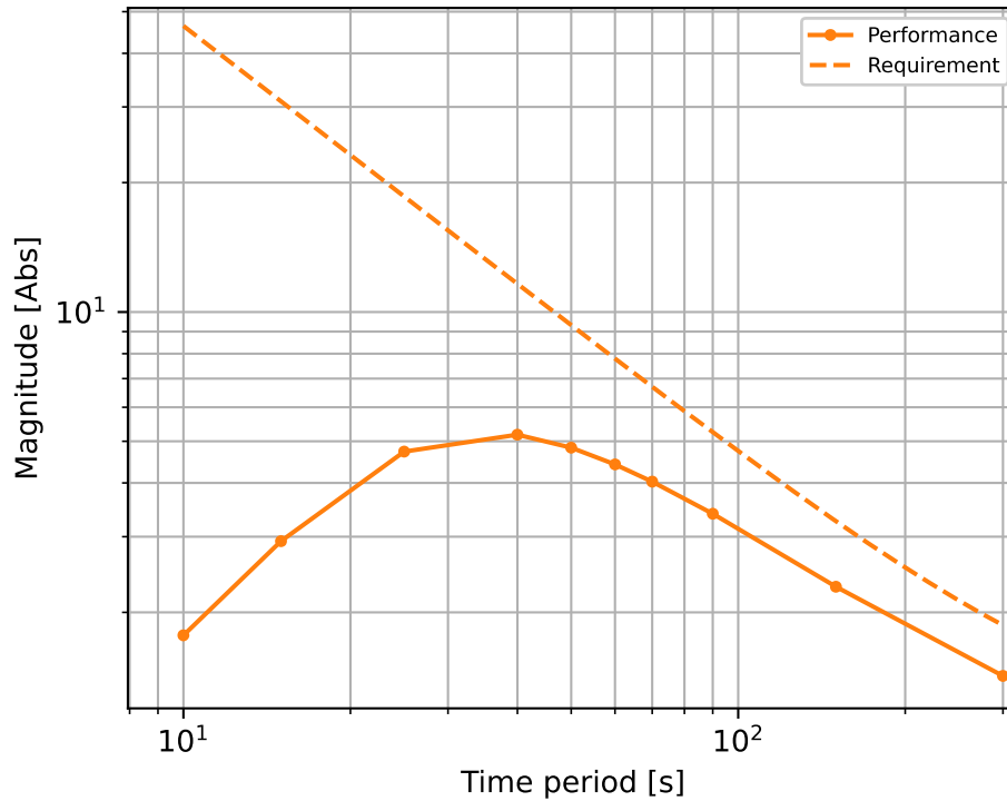
Figure 9. Example response of transfer function values (orange dots), interpolated transfer function (orange solid line) of the closed loop response, which qualifies for the performance requirement (orange dashed line). The dashed line shows the requirement for FCR-N.
