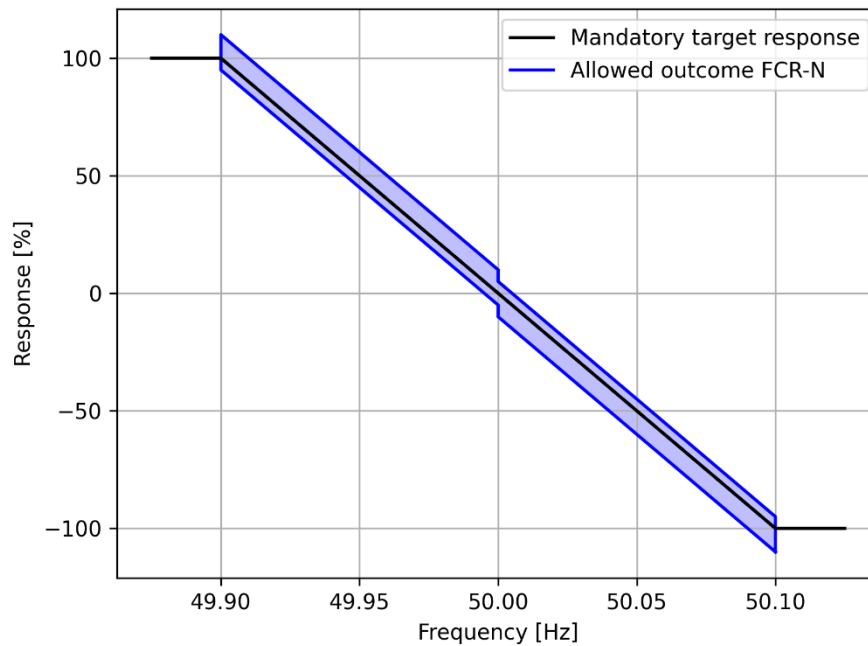
Figure 11. Activation of piecewise linear FCR-N resources. The black line indicates the mandatory target response. The controller shall be designed to minimise the deviation from the target response. The blue area defines the allowed outcome of the deviations, due to e.g. non-linear effects or step sizes for relay connected loads. The coordinates of the corners are provided in Table 1 below.
