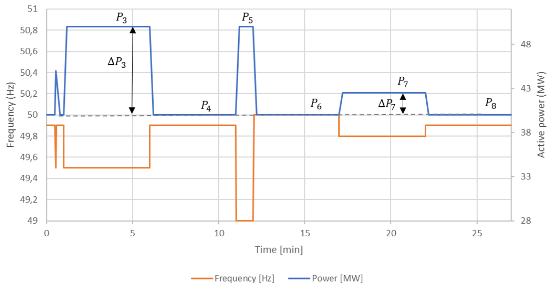
Figure 3. Illustration of FCR-D upwards ramp test. Here, FCR-N is inactive and therefore P_8 = P_6 .
