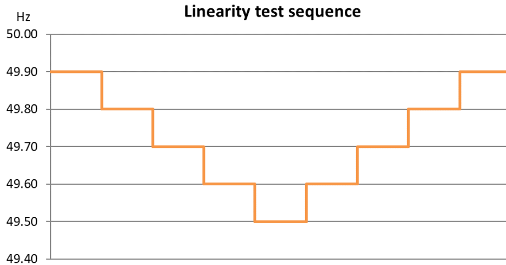
Figure 15. Grid frequency test signal for the FCR-D upwards linearity test.
