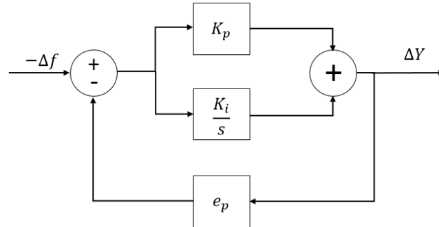
Figure 27. PI controller with droop where the K_p and K_i parameters are independent.
