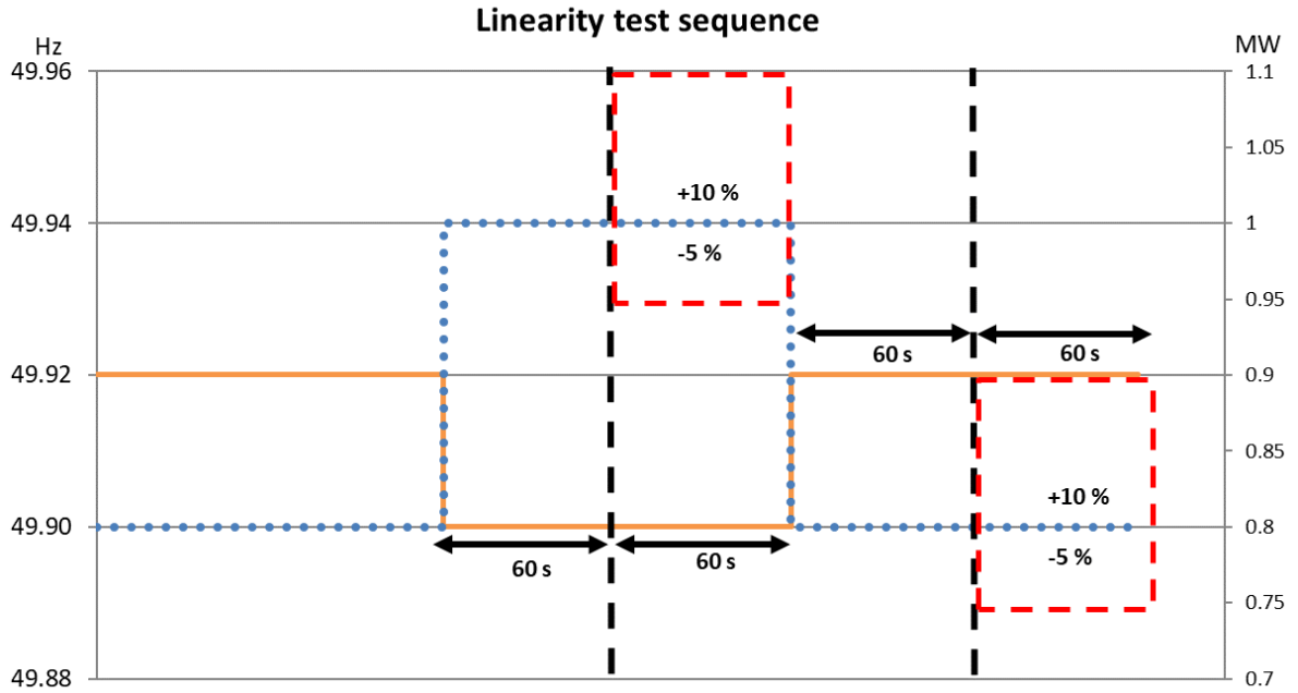
Figure 13. Allowed response area for FCR-N for the frequency steps from 49.92 Hz → 49.90 Hz → 49.92 Hz. The orange line is the frequency step. The blue dotted line is the directly proportional FCR response. The red dashed squares indicate the allowed response area.
