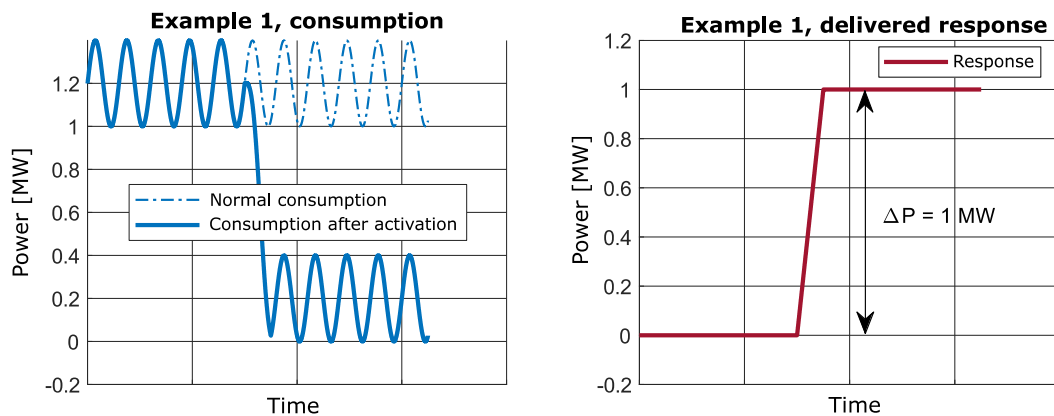
Figure 21. Example response where variations are independent of the delivered response.
