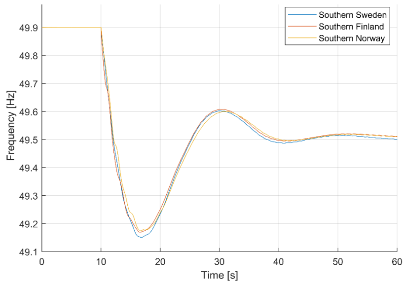
FIGURE 75: FREQUENCY RESPONSE FOR CASE 1 WHEN THE DISTURBANCE OCCUR AT DIFFERENT LOCATIONS, PARAMETER SET 1, FREQUENCY DEPENDENCY: ON, VOLTAGE DEPENDENCY: ON, PSS: ON.
