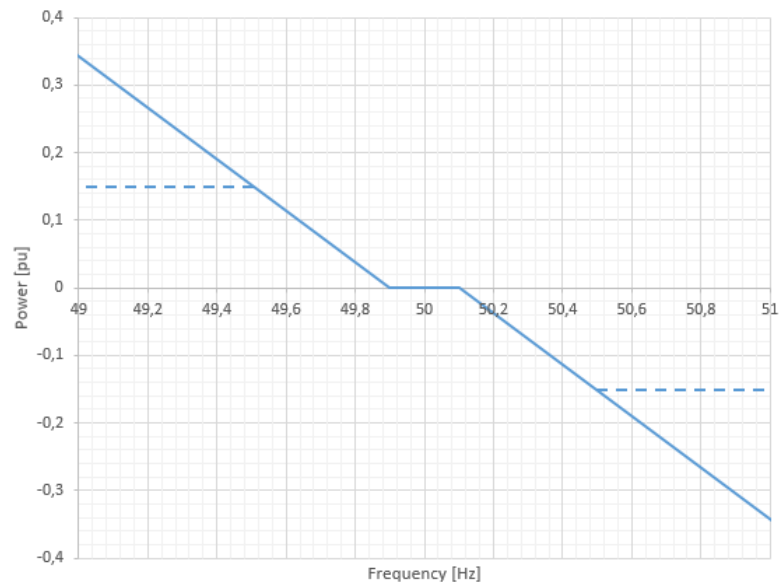
FIGURE 16: RELATION BETWEEN STEADY STATE POWER RESPONSE AND FREQUENCY DEVIATION FOR A SINGLE UNIT DELIVERING FCR-D. DASHED LINE IS SATURATION, WHICH IS ALLOWED AT FREQUENCIES <49.5 AND >50.5 Hz WITHOUT ADDITIONAL CONSIDERATIONS NECESSARY FOR STABILITY REQUIREMENT.
