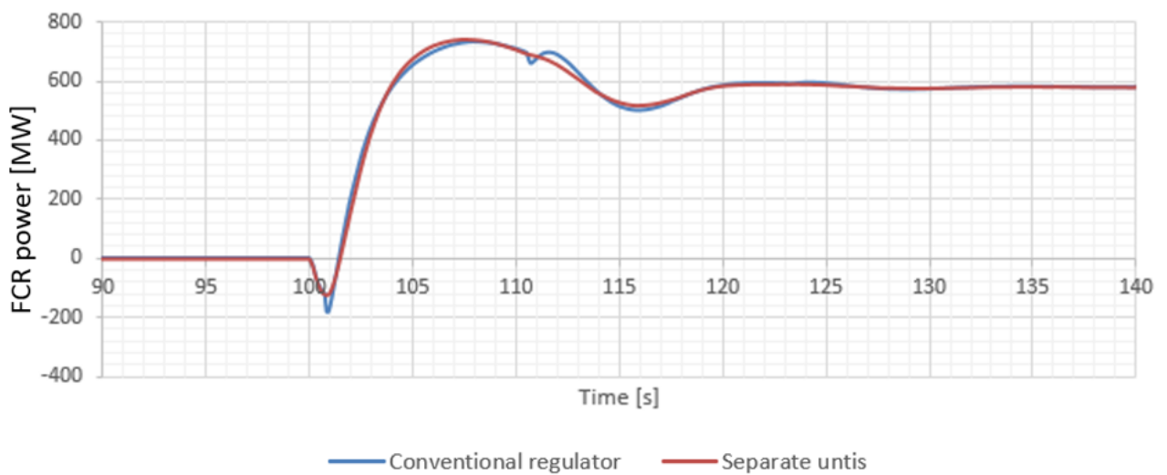
FIGURE 50 FCR POWER RESPONSE AFTER A 600 MW POWER STEP IN A SYSTEM WITH SEPARATE UNITS SUPPLYING FCR-N AND -D (ORANGE), AND A CONVENTIONAL REGULATOR SUPPLYING BOTH FCR-N AND -D (BLUE). PARAMETERS FROM TABLE 6, TABLE 7 AND TABLE 8, K_{D,FCR-N} = 0 AND K_{D,FCR-D} = 8 .
