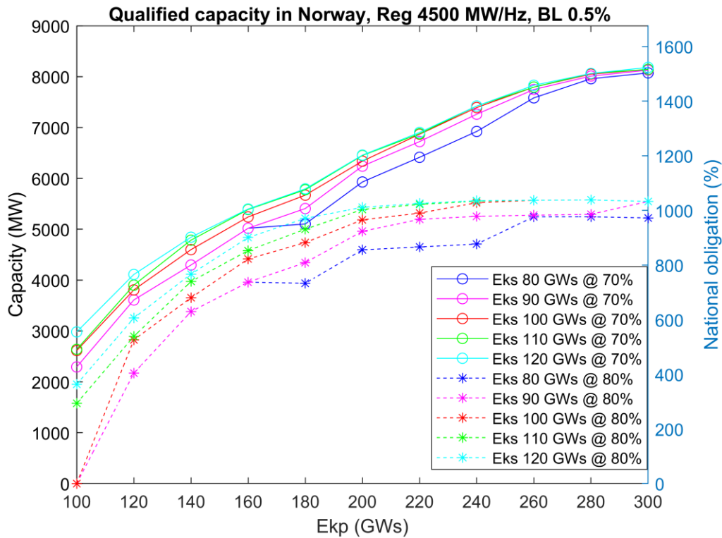
FIGURE 7. ESTIMATED CAPACITY IN NORWAY BASED ON INSTALLED CAPACITY AND DISTRIBUTION OF WATER TIME CONSTANTS. LEFT Y-AXIS IS IN MW AND TO THE RIGHT IN PERCENTAGE OF NATIONAL OBLIGATION (537 MW [FCR MARKET LIQUIDITY NEEDS]). BACKLASH IS SET TO 0.5 % OF RATED MACHINE POWER. EVALUATED FOR LOADING OF 70 % AND 80 %.
