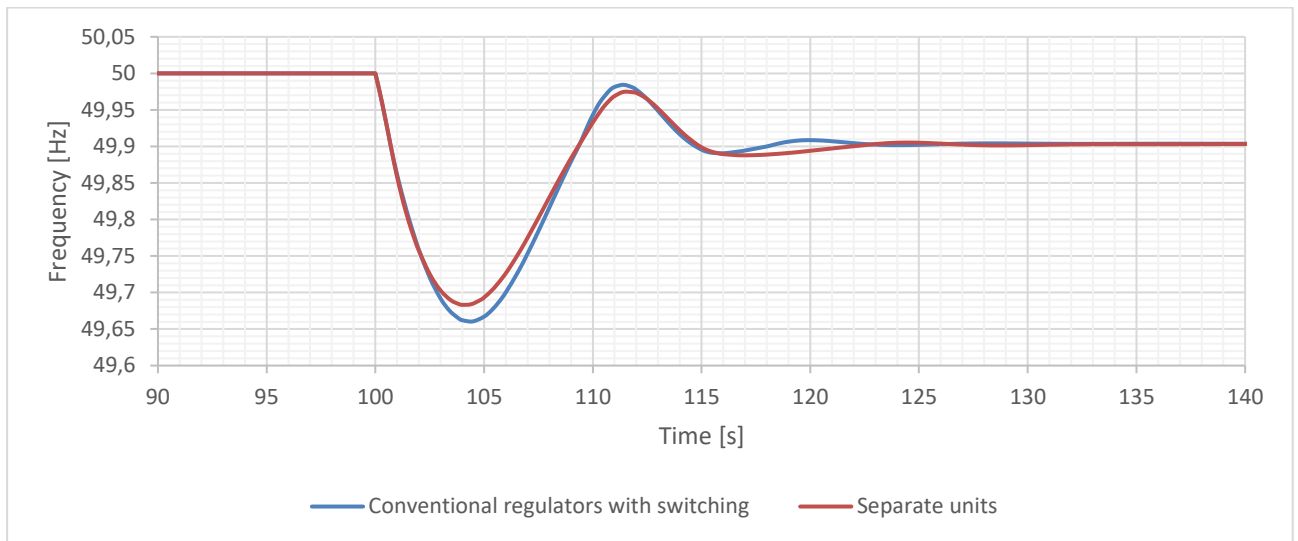
FIGURE 43 FREQUENCY RESPONSE AFTER A 600 MW POWER STEP FOR A SYSTEM WITH SEPARATE UNITS SUPPLYING FCR-N AND -D (ORANGE), AND A SYSTEM WITH A SHARE OF FCR UNITS HAVING CONVENTIONAL REGULATOR SUPPLYING BOTH FCR-N AND -D (BLUE). PARAMETERS FROM TABLE 6, TABLE 7 AND TABLE 8, BUT WITH K_{p,FCR-D} = 4.436 AND K_{p,FCR-N} = 10.436 .
