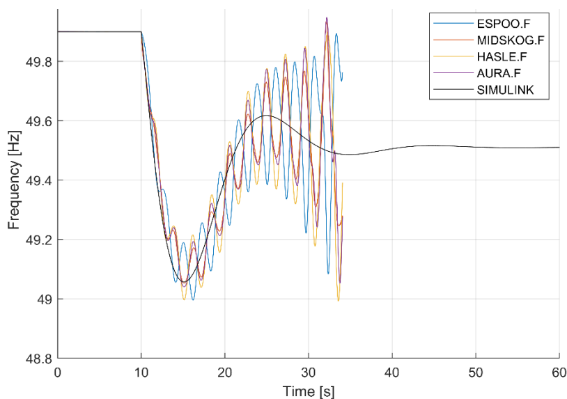
FIGURE 66: FREQUENCY RESPONSE COMPARISON FOR CASE 1, PARAMETER SET 1, DISTURBANCE: SOUTHERN SWEDEN, FREQUENCY DEPENDENCY: ON, VOLTAGE DEPENDENCY: ON, PSS: OFF.
