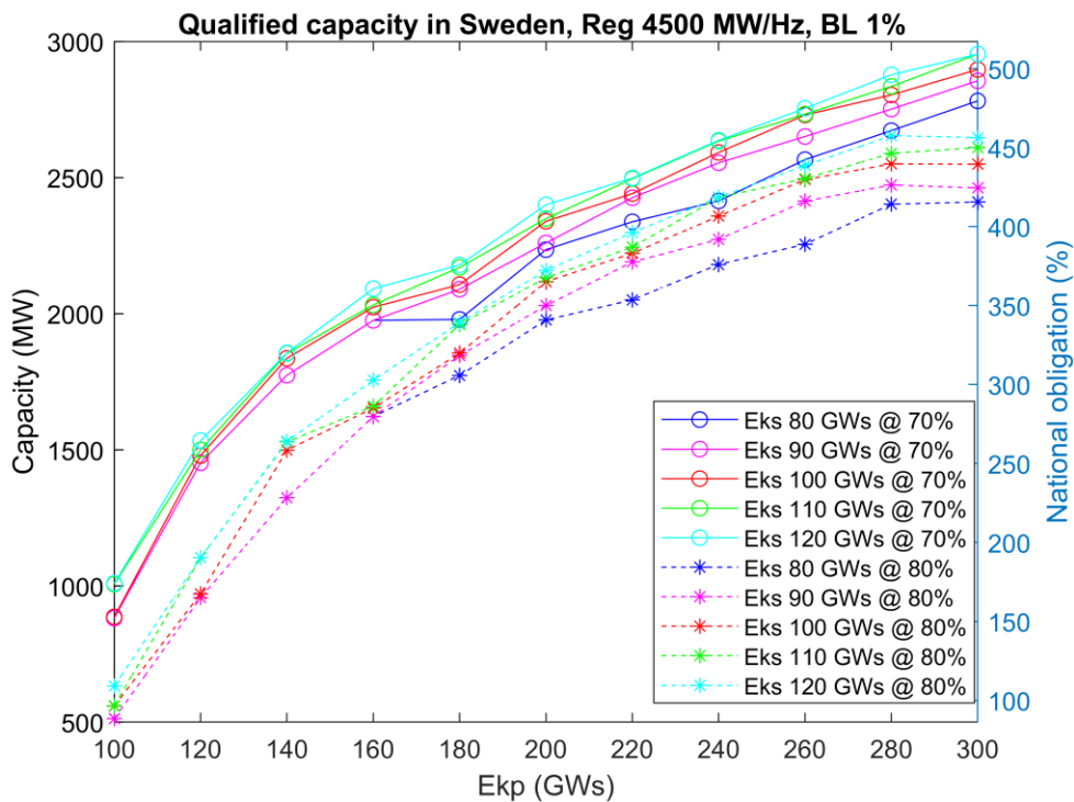
FIGURE 10. ESTIMATED CAPACITY IN SWEDEN BASED ON INSTALLED CAPACITY AND DISTRIBUTION OF WATER TIME CONSTANTS. LEFT Y-AXIS IS IN MW AND TO THE RIGHT IN PERCENTAGE OF NATIONAL OBLIGATION (580 MW [FCR MARKET LIQUIDITY NEEDS]). BACKLASH IS SET TO 1 % OF RATED MACHINE POWER. EVALUATED FOR LOADING OF 70 % AND 80 %.
