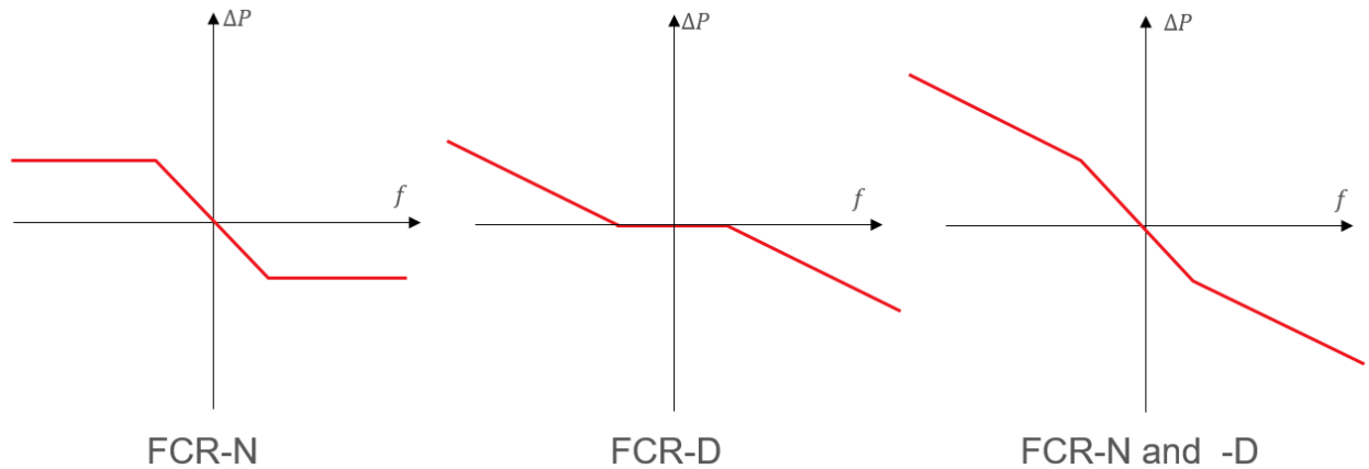
FIGURE 38 STEADY STATE RELATIONSHIP, DROOP PROFILE, OF A REGULATOR WITH PARALLEL STRUCTURE.
