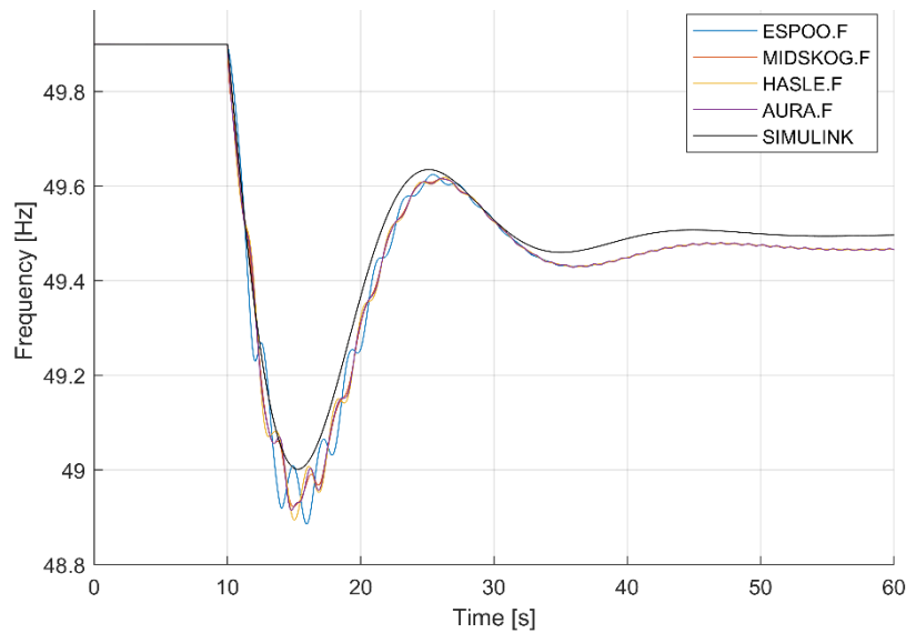
FIGURE 71: FREQUENCY RESPONSE COMPARISON FOR CASE 1, PARAMETER SET 1, DISTURBANCE: SOUTHERN SWEDEN, FREQUENCY DEPENDENCY: OFF, VOLTAGE DEPENDENCY: OFF, PSS: ON.
