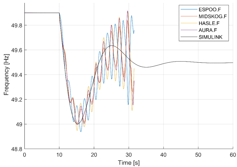
FIGURE 70: FREQUENCY RESPONSE COMPARISON FOR CASE 1, PARAMETER SET 1, DISTURBANCE: SOUTHERN SWEDEN, FREQUENCY DEPENDENCY: OFF, VOLTAGE DEPENDENCY: ON, PSS: OFF.
