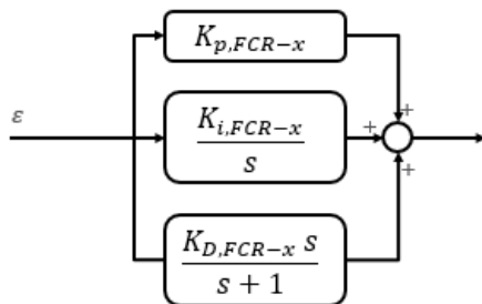
FIGURE 32 PID-STRUCTURE AND PARAMETERS NOTATION. THE FCR-X REFERS TO EITHER PARAMETER SET FOR FCR-N OR -D.
