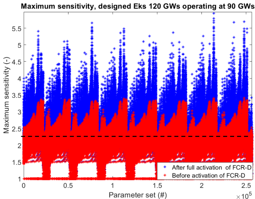
FIGURE 15. CLOSE LOOP STABILITY AT 120 GWs ASSESSED AT 90 GWs. THE BLACK DASHED LINE INDICATES THE DESIGNED MAXIMUM SENSITIVITY (2.31) AT 120 GWs.
