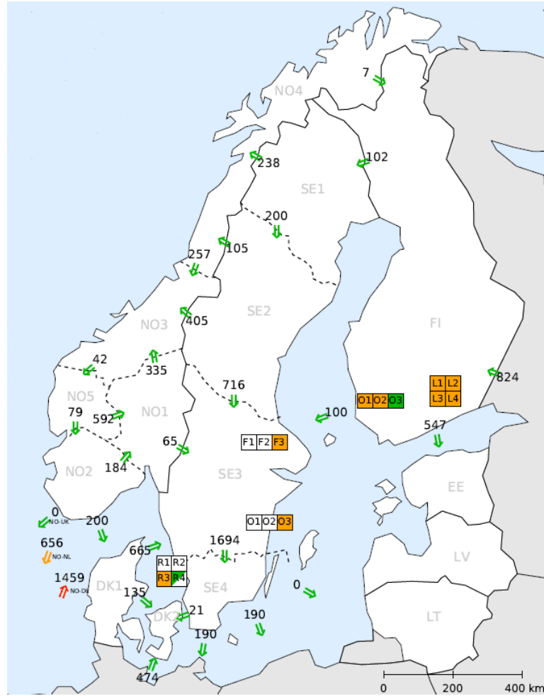
FIGURE 63: ACTIVE POWER FLOWS IN CASE 1. THE VALUES ARE IN MW.
