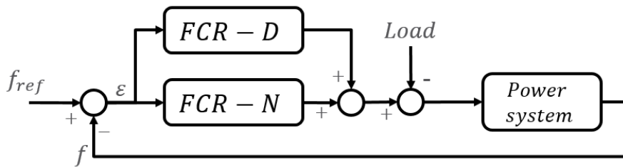
FIGURE 29 MODEL OF A SYSTEM WITH FCR-N AND -D SUPPLIED SEPARATELY.
