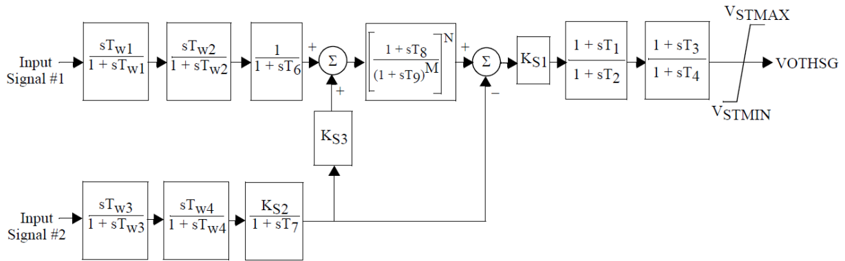
FIGURE 57: COMMONLY USED POWER SYSTEM STABILISER (PSS) MODEL PSS2A IN THE NORDIC PSS/E SIMULATION MODEL [PSS/E 33.9 MODEL LIBRARY].
