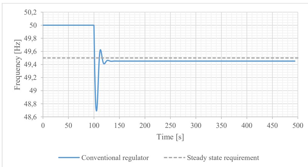
FIGURE 35 FREQUENCY RESPONSE OF A SYSTEM WITH A CONVENTIONAL REGULATOR SWITCHING BETWEEN e_{p,FCR-N} = 0.04 AND e_{p,FCR-D} = 0.08 . THE IMPOSED POWER IMBALANCE IS 2050 MW.
