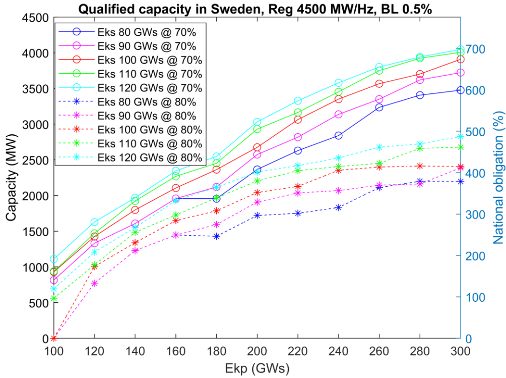
FIGURE 9. ESTIMATED CAPACITY IN SWEDEN BASED ON INSTALLED CAPACITY AND DISTRIBUTION OF WATER TIME CONSTANTS. LEFT Y-AXIS IS IN MW AND TO THE RIGHT IN PERCENTAGE OF NATIONAL OBLIGATION (580 MW [FCR MARKET LIQUIDITY NEEDS]). BACKLASH IS SET TO 0.5 % OF RATED MACHINE POWER. EVALUATED FOR LOADING OF 70 % AND 80 %.
