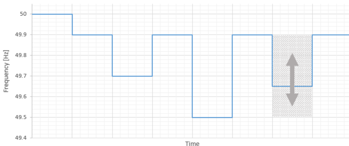
FIGURE 23: FCR-D UPWARDS REGULATION STEP RESPONSE SEQUENCE FOR UNITS SATURATING.
