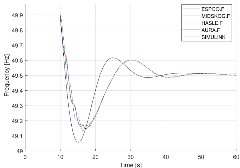
FIGURE 65: FREQUENCY RESPONSE COMPARISON FOR CASE 1, PARAMETER SET 1, DISTURBANCE: SOUTHERN SWEDEN, FREQUENCY DEPENDENCY: ON, VOLTAGE DEPENDENCY: ON, PSS: ON.
