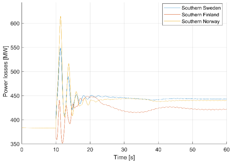
FIGURE 77: ACTIVE POWER LOSSES FOR CASE 1 WHEN THE DISTURBANCE OCCUR AT DIFFERENT LOCATIONS, PARAMETER SET 1, FREQUENCY DEPENDENCY: ON, VOLTAGE DEPENDENCY: ON, PSS: ON.
