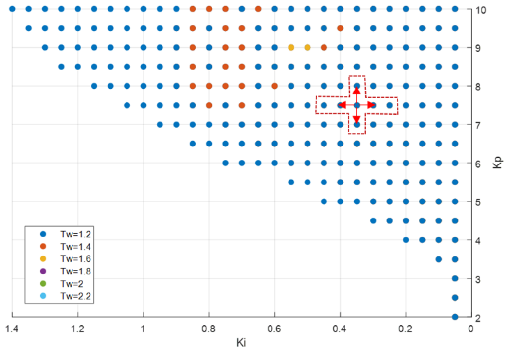
FIGURE 5: QUALIFIED PARAMETER SETS AS A FUNCTION OF PROPORTIONAL GAIN, K_p , AND INTEGRAL GAIN, K_i , FOR DIFFERENT WATER TIME CONSTANTS, T_w (SEE LEGEND). 2D-VISUALISATION OF FIGURE 4. EKS=90 GWS, EKP=300 GWS, BACKLASH=0.5% AND DROOP AT 4%.
