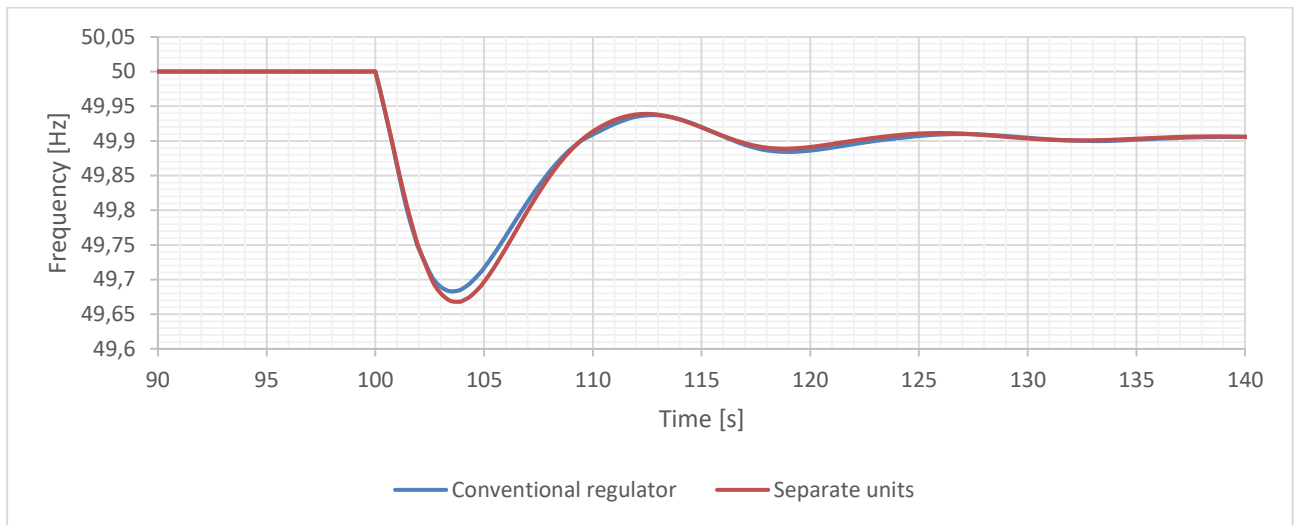
FIGURE 41 FREQUENCY RESPONSE AFTER A 600 MW POWER STEP FOR A SYSTEM WITH SEPARATE UNITS SUPPLYING FCR-N AND -D (ORANGE), AND A SYSTEM WITH A SHARE OF FCR UNITS HAVING CONVENTIONAL REGULATOR SUPPLYING BOTH FCR-N AND -D (BLUE). PARAMETERS FROM TABLE 6, TABLE 7 AND TABLE 8, BUT WITH K_{p,FCR-N} = 4.436 AND K_{p,FCR-D} = 10.436 .
