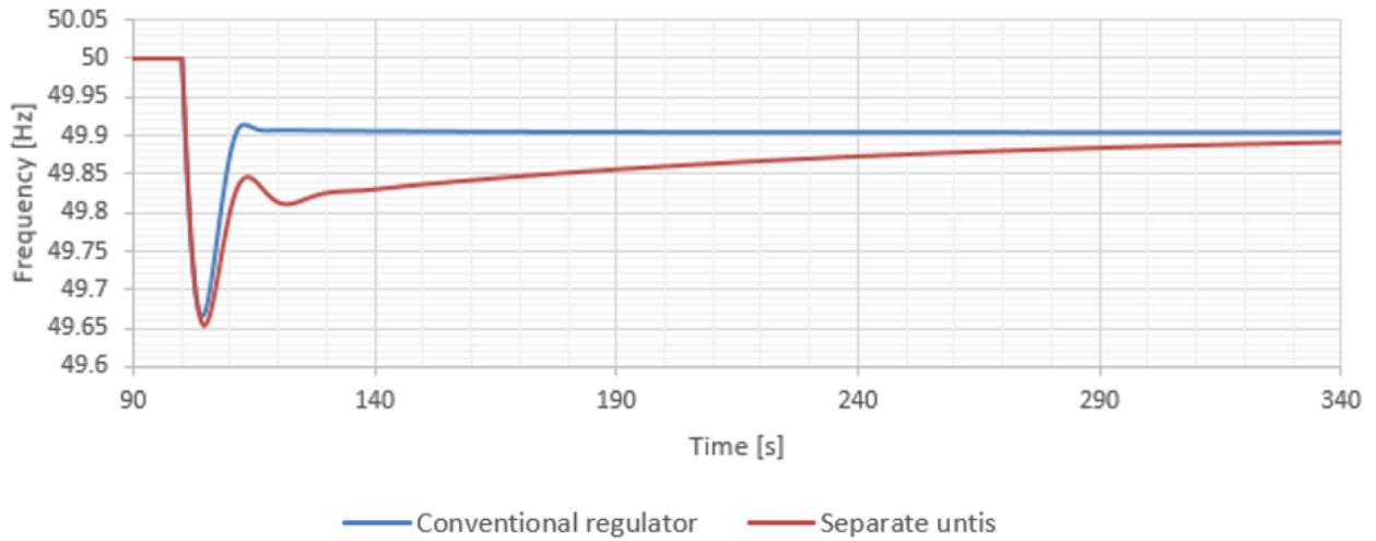
FIGURE 47 FREQUENCY RESPONSE AFTER A 600 MW POWER STEP IN A SYSTEM WITH SEPARATE UNITS SUPPLYING FCR-N AND -D (ORANGE) AND A CONVENTIONAL REGULATOR SUPPLYING BOTH FCR-N AND -D (BLUE). PARAMETERS TABLE 6, TABLE 7 AND TABLE 8, BUT WITH K_{i,FCR-D} = 0.2 AND K_{i,FCR-N} = 4 .
