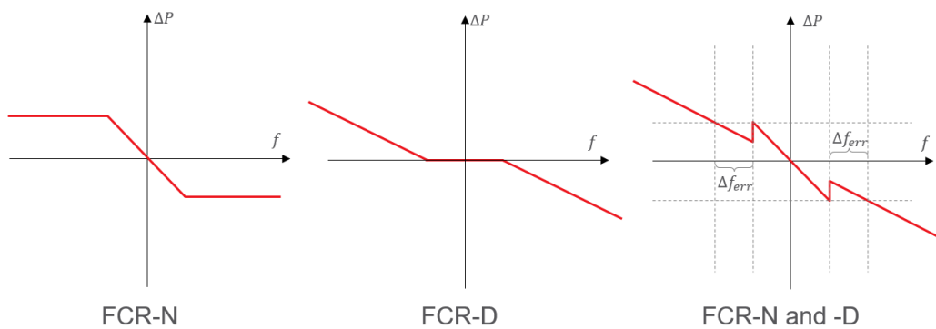
FIGURE 34 STEADY STATE RELATIONSHIP BETWEEN POWER CHANGE AND FREQUENCY DEVIATION (DROOP PROFILE) OF A CONVENTIONAL REGULATOR WITH SWITCHING OF DROOP AT A THRESHOLD ( e_{p,FCR-N} < e_{p,FCR-D} )
