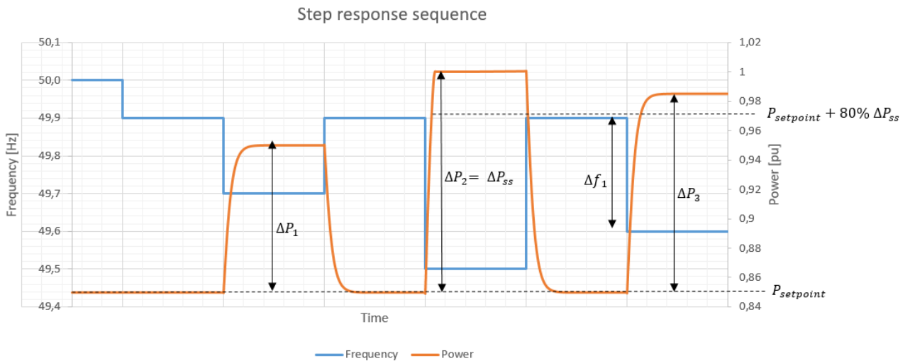
FIGURE 22: EXAMPLE OF PREQUALIFICATION TEST TO DETERMINE THE SATURATION FACTOR
