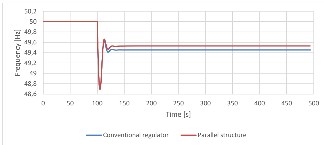
FIGURE 39 FREQUENCY RESPONSE OF A SYSTEM WITH CONVENTIONAL REGULATOR STRUCTURE (BLUE) AND PARALLEL REGULATOR STRUCTURE (RED), SWITCHING BETWEEN e_{p,FCR-N} = 0.04 AND e_{p,FCR-D} = 0.08 . THE POWER IMBALANCE IS 2050 MW.
