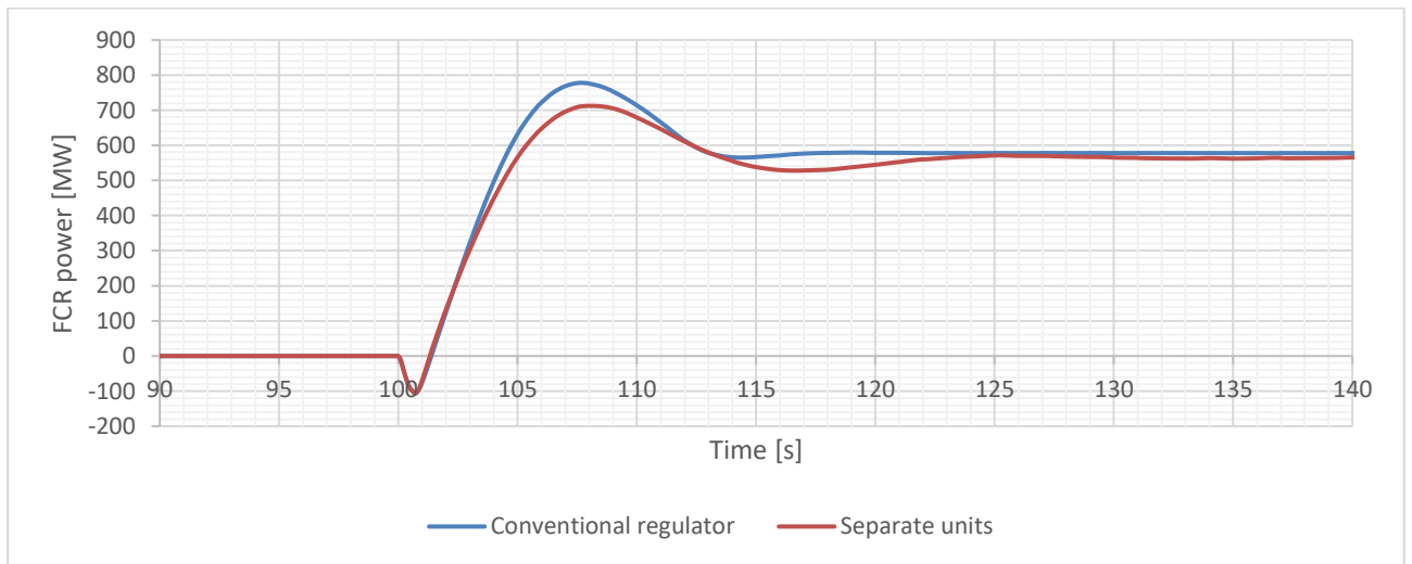
FIGURE 46 FCR POWER RESPONSE AFTER A 600 MW POWER STEP IN A SYSTEM WITH SEPARATE UNITS SUPPLYING FCR-N AND -D (ORANGE), AND A CONVENTIONAL REGULATOR SUPPLYING BOTH FCR-N AND -D (BLUE). PARAMETERS FROM TABLE 6, TABLE 7 AND TABLE 8, BUT WITH K_{i,FCR-N} = 0.2 AND K_{i,FCR-D} = 4 .
