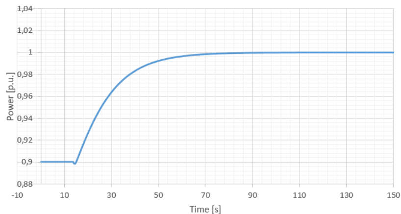
FIGURE 17: EXAMPLE OF A -0.4 Hz STEP RESPONSE FOR A UNIT RUNNING THE TEST FOR DOCUMENTING THE STEADY STATE DELIVERY OF FCR-D
