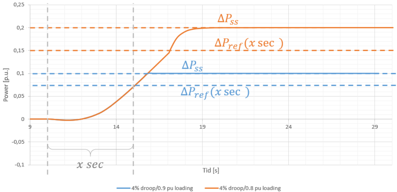
FIGURE 19: FCR UNIT RESPONSE ON PERFORMANCE WITH SATURATION WITHIN THE FCR-D FREQUENCY BAND OF 49.5-50.5 Hz (BLUE) AND WITHOUT SATURATION WITHIN THE FCR-D FREQUENCY BAND (ORANGE). THE UNIT IS IDENTICAL BETWEEN THE TWO RESPONSES, EXCEPT SETPOINT.
