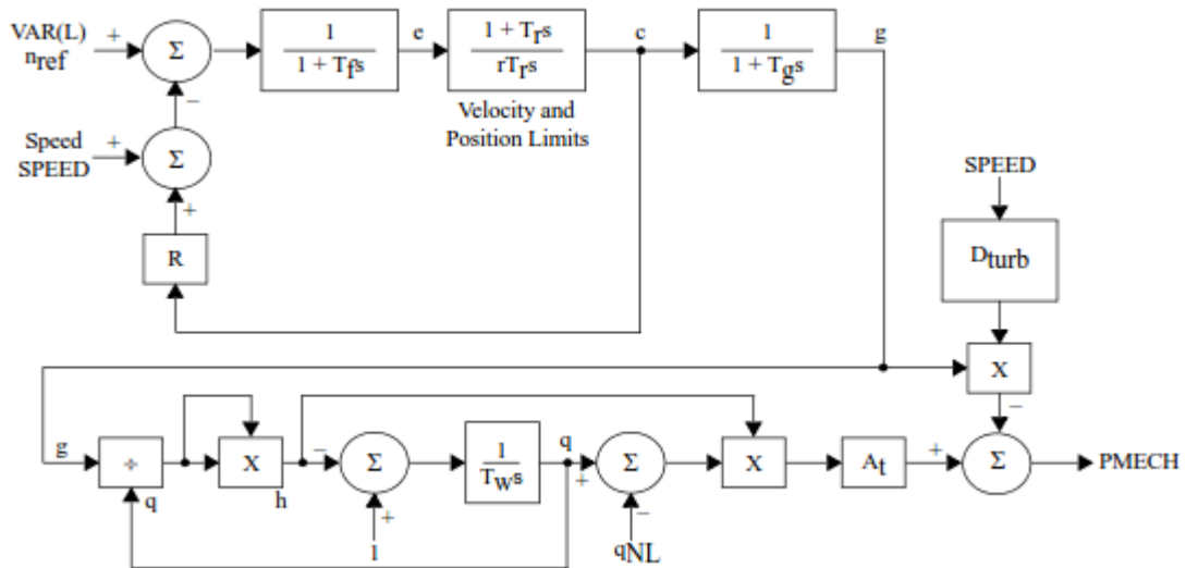
FIGURE 58: HYGOV TURBINE GOVERNOR MODEL [PSS/E 33.8 MODEL LIBRARY].
