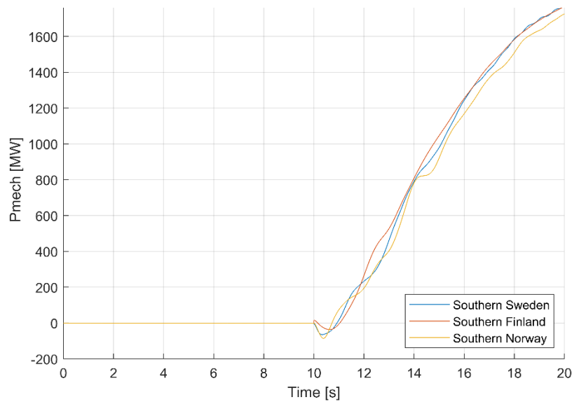
FIGURE 79: MECHANICAL POWER OF FCR FOR CASE 1, PARAMETER SET 1, FREQUENCY DEPENDENCY: ON, VOLTAGE DEPENDENCY: ON, PSS: ON.
