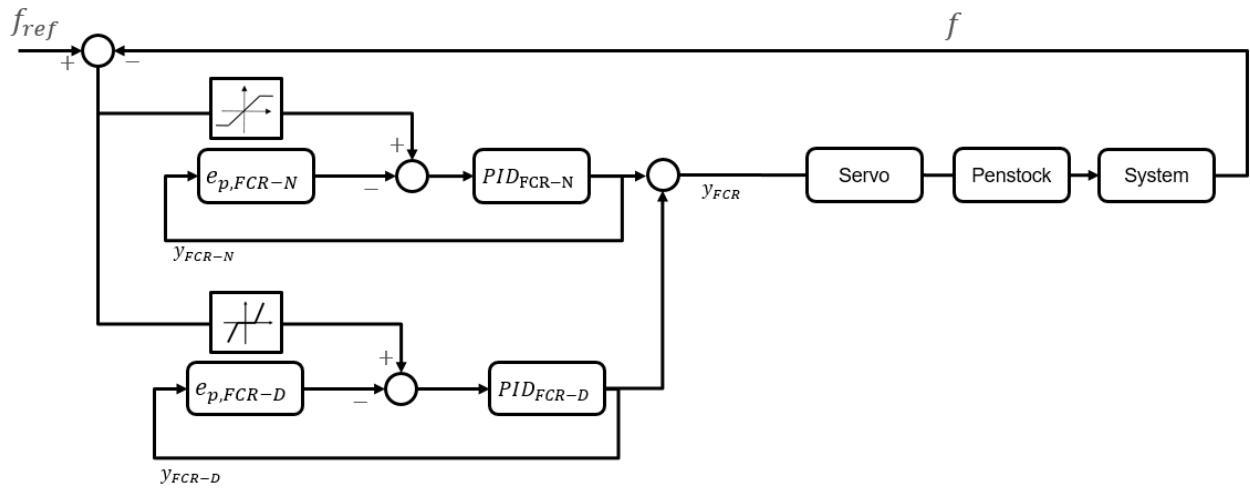
FIGURE 33 SCHEMATIC (SIMPLIFIED) FREQUENCY CONTROL WITH PID FEEDBACK AND PARALLEL REGULATORS FOR FCR-N AND -D.
