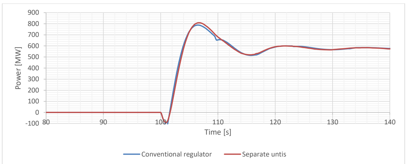
FIGURE 42 FCR UNITS POWER RESPONSE AFTER A 600 MW POWER STEP FOR A SYSTEM WITH SEPARATE UNITS SUPPLYING FCR-N AND -D (ORANGE), AND A SYSTEM WITH A SHARE OF UNITS HAVING CONVENTIONAL REGULATOR SUPPLYING BOTH FCR-N AND -D (BLUE). PARAMETERS FROM TABLE 6, TABLE 7 AND TABLE 8, BUT WITH K_{p,FCR-N} = 4.436 AND K_{p,FCR-D} = 10.436 .
