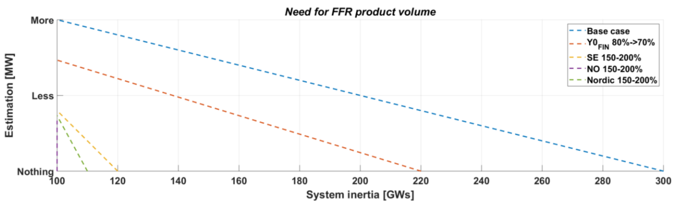
FIGURE 25. OVERVIEW – NEED OF FAST FREQUENCY RESERVE (FFR) AS A CHOICE OF FCR-D KINETIC ENERGY FOR PERFORMANCE.
