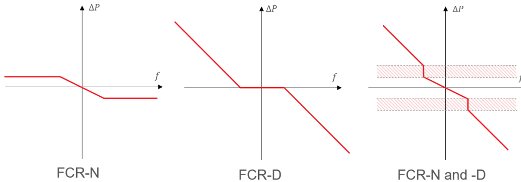
FIGURE 36 STEADY STATE RELATIONSHIP BETWEEN POWER CHANGE AND FREQUENCY DEVIATION (DROOP PROFILE) FOR A CONVENTIONAL REGULATOR WITH SWITCHING OF DROOP AT A THRESHOLD ( e_{p,FCR-N} > e_{p,FCR-D} ).
