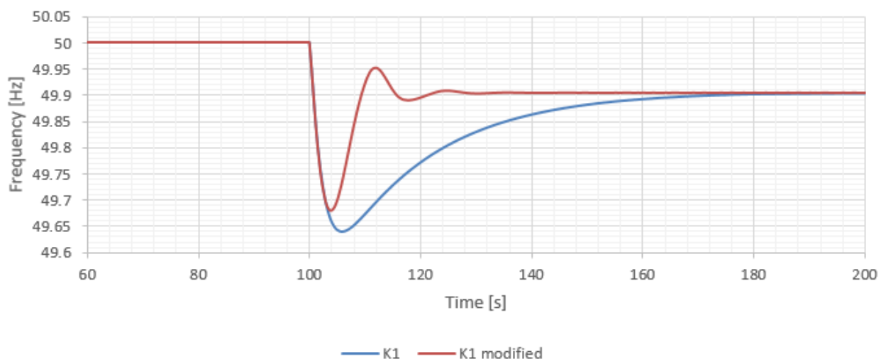
FIGURE 27 EFFECT OF MODIFYING THE K1 PARAMETER SET TO GET OSCILLATIONS IN THE SYSTEM.
