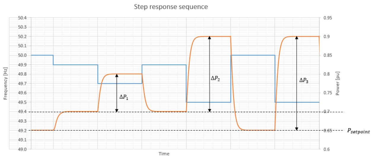
FIGURE 55 EXAMPLE OF STEP RESPONSE FOR FCR-D UPWARDS REGULATION FOR DELIVERING BOTH FCR-N AND FCR-D
