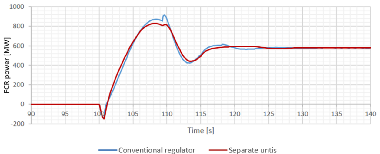
FIGURE 44 FCR UNITS POWER RESPONSE AFTER A 600 MW POWER STEP FOR A SYSTEM WITH SEPARATE UNITS SUPPLYING FCR-N AND -D (ORANGE), AND A SYSTEM WITH A SHARE OF UNITS HAVING CONVENTIONAL REGULATOR SUPPLYING BOTH FCR-N AND -D (BLUE). PARAMETERS FROM TABLE 6, TABLE 7 AND TABLE 8, BUT WITH K_{p,FCR-D} = 4.436 AND K_{p,FCR-N} = 10.436 .
