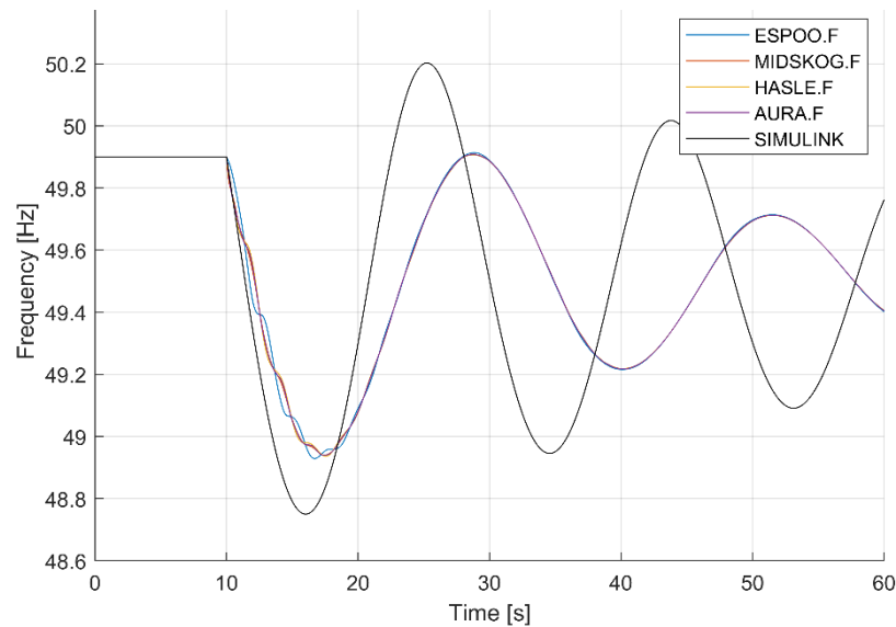
FIGURE 73: FREQUENCY RESPONSE COMPARISON FOR CASE 1, PARAMETER SET 2, DISTURBANCE: SOUTHERN SWEDEN, FREQUENCY DEPENDENCY: ON, VOLTAGE DEPENDENCY: ON, PSS: ON.
