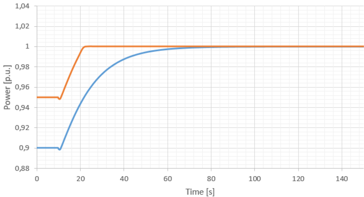
FIGURE 18: EXAMPLE OF A -0.4 Hz STEP RESPONSE FOR A UNIT RUNNING THE TEST FOR DOCUMENTING THE STEADY STATE DELIVERY OF FCR-D, BUT WITH SATURATION DUE TO MAXIMUM POWER BEING REACHED.
