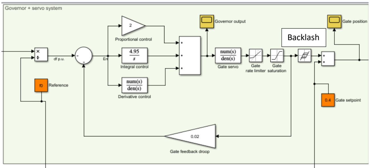
FIGURE 6. BLOCK DIAGRAM OF THE GOVERNOR AND SERVO.
