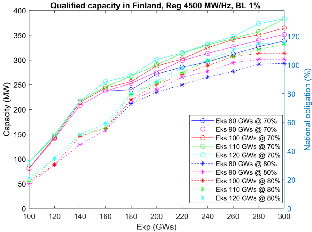
FIGURE 12. ESTIMATED CAPACITY IN FINLAND BASED ON INSTALLED CAPACITY AND DISTRIBUTION OF WATER TIME CONSTANTS. LEFT Y-AXIS IS IN MW AND TO THE RIGHT IN PERCENTAGE OF NATIONAL OBLIGATION (290 MW [FCR MARKET LIQUIDITY NEEDS]). BACKLASH IS SET TO 1 % OF RATED MACHINE POWER.
