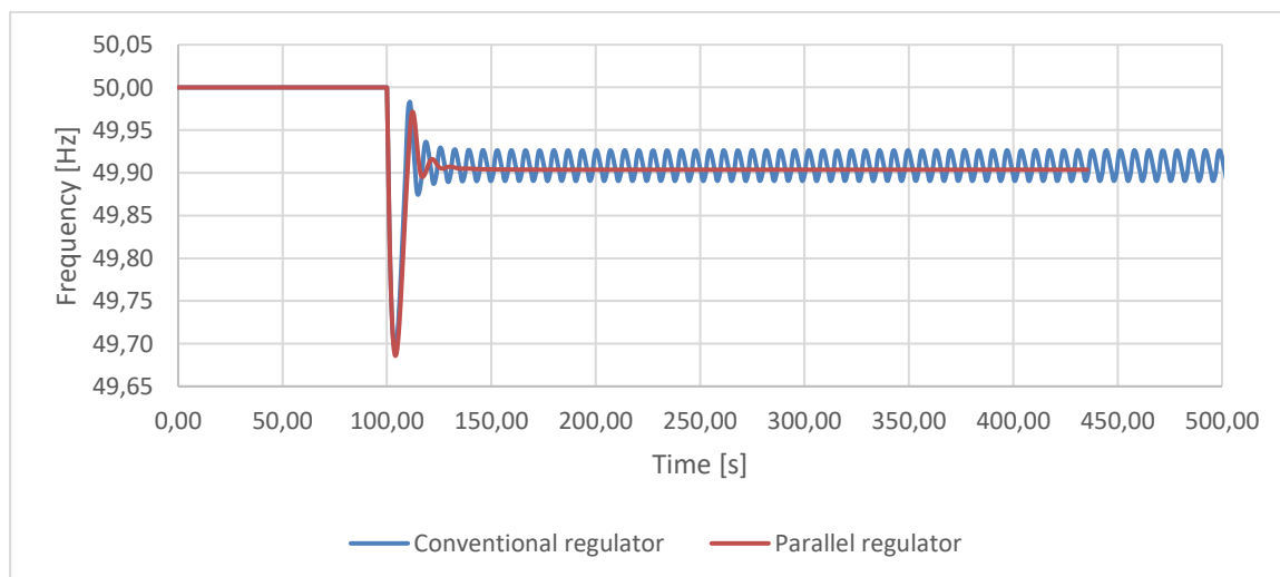
FIGURE 40 FREQUENCY RESPONSE OF A SYSTEM WITH CONVENTIONAL REGULATOR STRUCTURE (BLUE) AND PARALLEL REGULATOR STRUCTURE (RED), SWITCHING BETWEEN e_{p,FCR-N} = 0.08 AND e_{p,FCR-D} = 0.04 . THE POWER IMBALANCE IS 600 MW.
