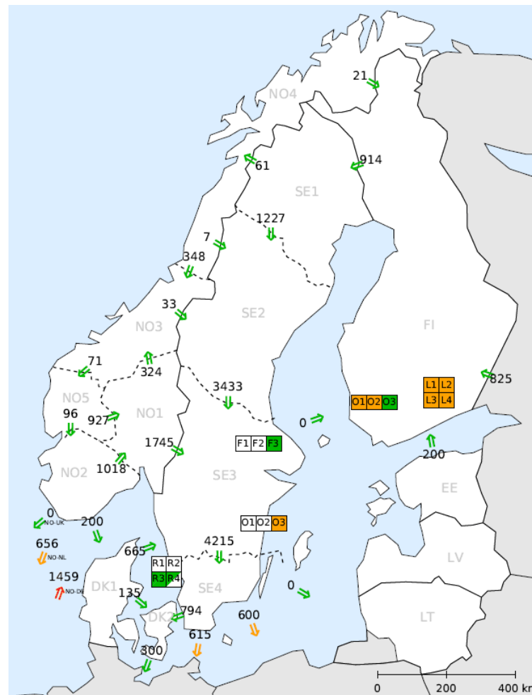
FIGURE 64: ACTIVE POWER FLOWS IN CASE 2. THE VALUES ARE IN MW.
