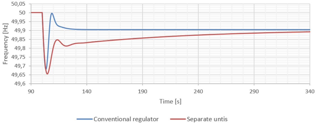
FIGURE 45 FREQUENCY RESPONSE AFTER A 600 MW POWER STEP IN A SYSTEM WITH SEPARATE UNITS SUPPLYING FCR-N AND -D (ORANGE) AND A CONVENTIONAL REGULATOR SUPPLYING BOTH FCR-N AND -D (BLUE). PARAMETERS FROM TABLE 6, TABLE 7 AND TABLE 8, BUT WITH K_{i,FCR-N} = 0.2 AND K_{i,FCR-D} = 4 .
