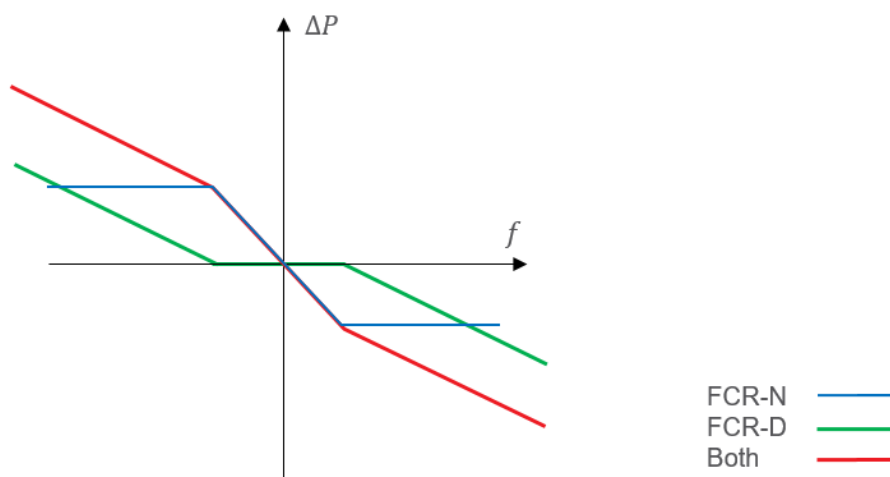
FIGURE 54 STEADY STATE ACTIVATION, DROOP PROFILE, OF FCR-N (BLUE), FCR-D (GREEN) AND BOTH (RED).
