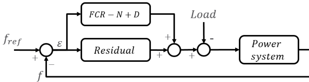
FIGURE 30 MODELLING A SYSTEM WITH FCR-N AND -D PARTLY SUPPLIED FROM UNITS DELIVERING BOTH FCR-N AND -D, AND THE RESIDUAL FCR DELIVERED FROM A PARALLEL BRANCH.
