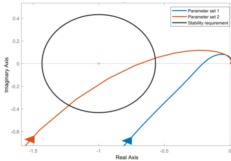
FIGURE 62: NYQUIST DIAGRAM FOR PARAMETER SET 1 AND 2 FOR A 120 GW SYSTEM
