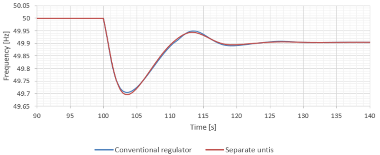
FIGURE 49 FREQUENCY RESPONSE AFTER A 600 MW POWER STEP IN A SYSTEM WITH SEPARATE UNITS SUPPLYING FCR-N AND -D (ORANGE), AND A CONVENTIONAL REGULATOR SUPPLYING BOTH FCR-N AND -D (BLUE). PARAMETERS FROM TABLE 6, TABLE 7 AND TABLE 8, BUT WITH K_{D,FCR-N} = 0 AND K_{D,FCR-D} = 8 .
