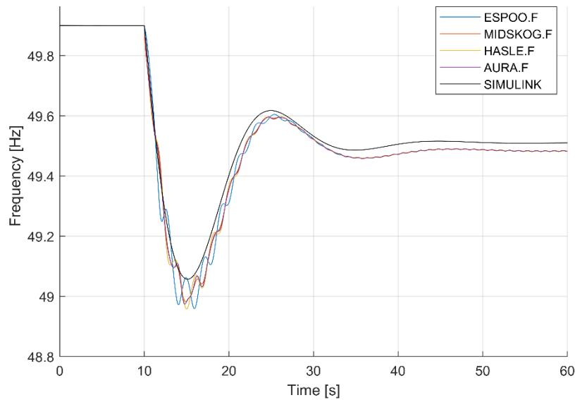
FIGURE 67: FREQUENCY RESPONSE COMPARISON FOR CASE 1, PARAMETER SET 1, DISTURBANCE: SOUTHERN SWEDEN, DEPENDENCY: ON, VOLTAGE DEPENDENCY: OFF, PSS: ON.
