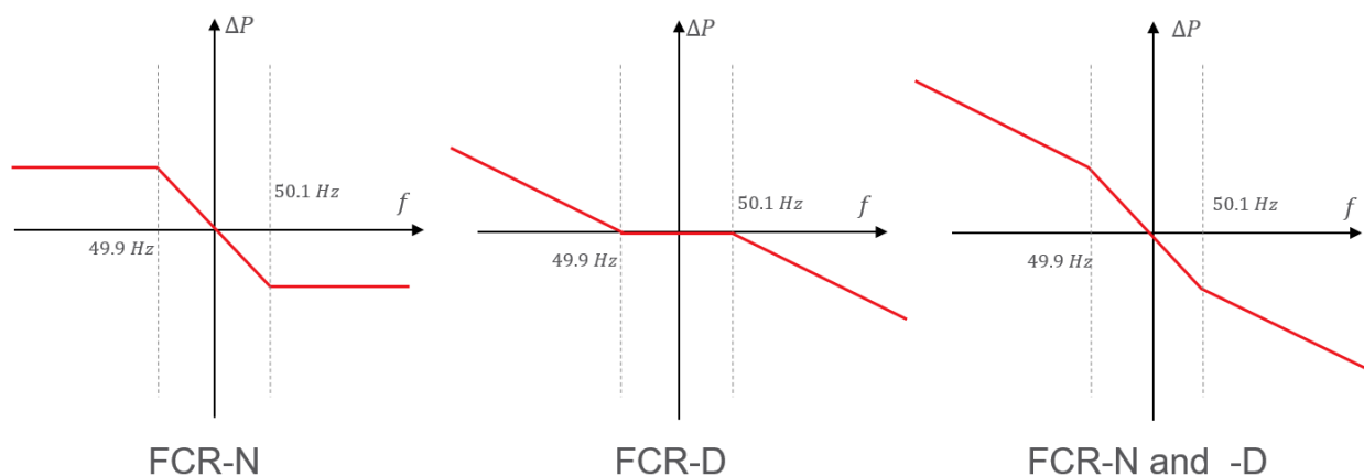
FIGURE 26: DROOP PROFILE ON SYSTEM LEVEL FOR FCR-N, FCR-D AND FOR THEM COMBINED.
