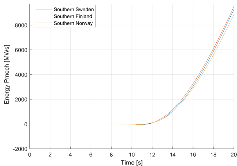
FIGURE 80: MECHANICAL ENERGY OF FCR FOR CASE 1, PARAMETER SET 1, FREQUENCY DEPENDENCY: ON, VOLTAGE DEPENDENCY: ON, PSS: ON.
