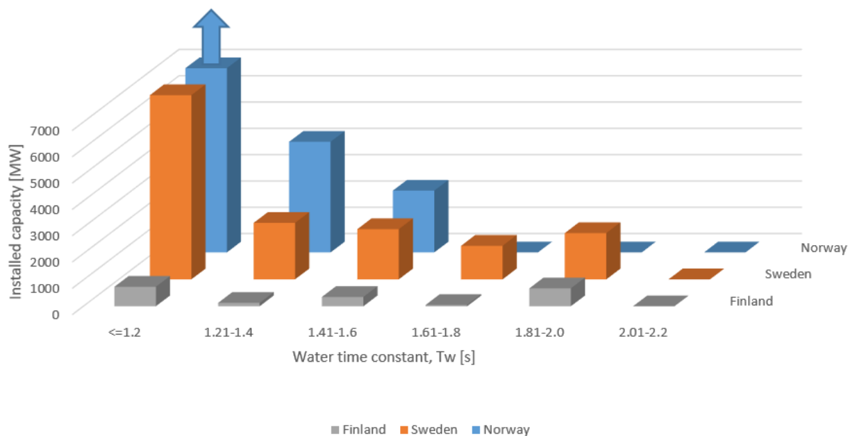
FIGURE 3: INSTALLED HYDRO CAPACITY IN THE NORDIC POWER SYSTEM DISTRIBUTED BY COUNTRY AND WATER TIME CONSTANT
