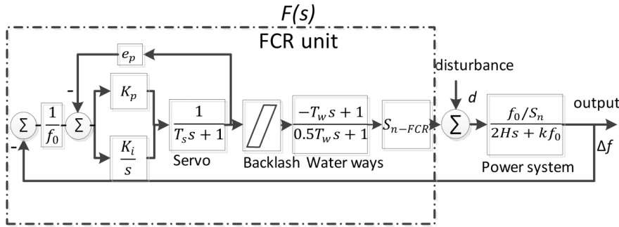
FIGURE 28 NON-LINEAR AGGREGATED REFERENCE MODEL.
