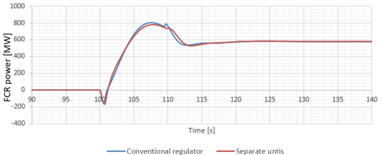
FIGURE 52 FCR POWER RESPONSE AFTER A 600 MW POWER STEP IN A SYSTEM WITH SEPARATE UNITS SUPPLYING FCR-N AND -D (ORANGE), AND A CONVENTIONAL REGULATOR SUPPLYING BOTH FCR-N AND -D (BLUE). PARAMETERS FROM TABLE 6, TABLE 7 AND TABLE 8, K_{D,FCR-N} = 8 AND K_{i,FCR-D} = 0 .
