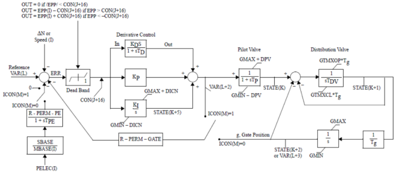
FIGURE 59: WEHGOV TURBINE GOVERNOR MODEL, GOVERNOR AND HYDRAULIC ACTUATORS PART [PSS/E 33.8 MODEL LIBRARY].
