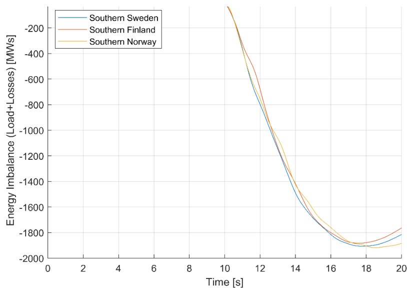
FIGURE 78: ENERGY OF LOAD AND LOSSES FOR CASE 1 WHEN THE DISTURBANCE OCCUR AT DIFFERENT LOCATIONS, PARAMETER SET 1, FREQUENCY DEPENDENCY: ON, VOLTAGE DEPENDENCY: ON, PSS: ON.
