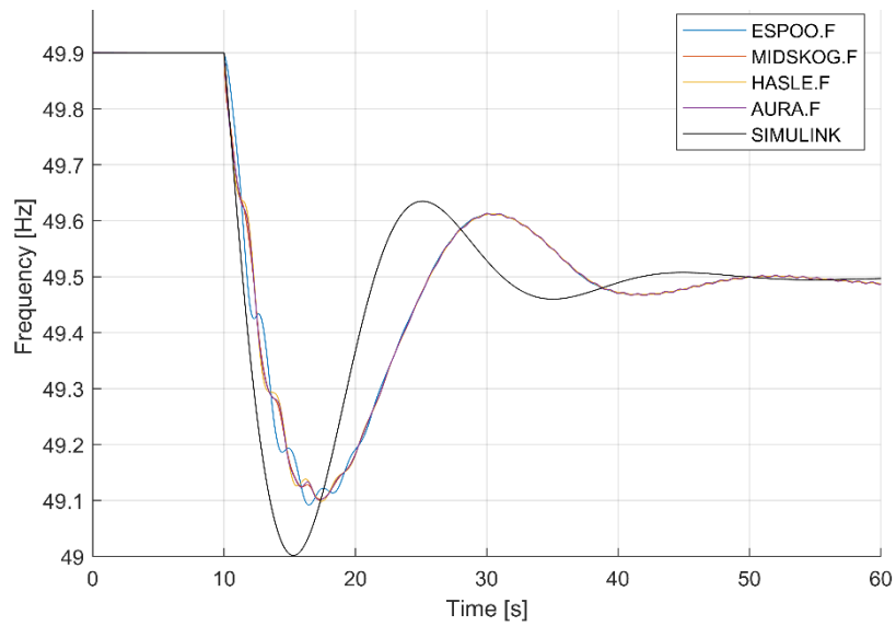
FIGURE 69: FREQUENCY RESPONSE COMPARISON FOR CASE 1, PARAMETER SET 1, DISTURBANCE: SOUTHERN SWEDEN, FREQUENCY DEPENDENCY: OFF, VOLTAGE DEPENDENCY: ON, PSS: ON.
