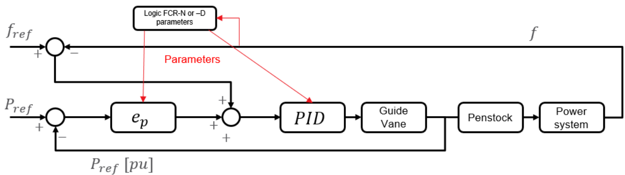
FIGURE 31 SCHEMATIC (SIMPLIFIED) FREQUENCY CONTROL SYSTEM WITH GATE FEEDBACK AND SWITCHING OF PARAMETERS AT THE FREQUENCY THRESHOLD.
