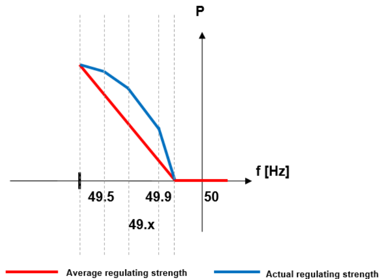
FIGURE 20: ILLUSTRATION OF NON-LINEAR RELATION BETWEEN STEADY STATE POWER RESPONSE AND FREQUENCY DEVIATION WITHIN THE FCR-D RANGE DUE TO SATURATION.
