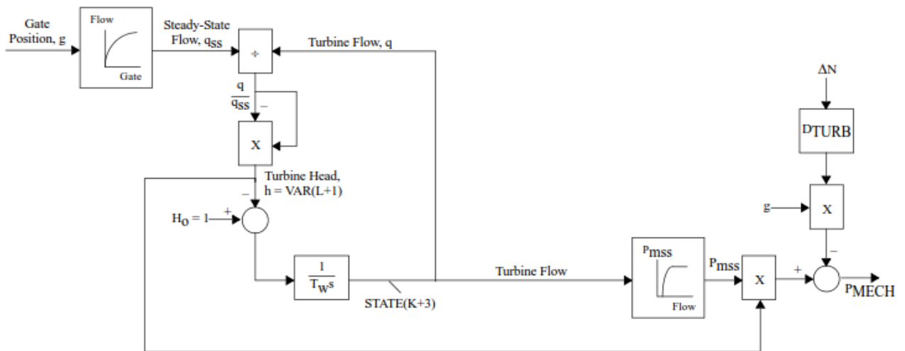
FIGURE 60: WEHGOV TURBINE GOVERNOR MODEL, TURBINE DYNAMICS PART [PSS/E 33.8 MODEL LIBRARY].
