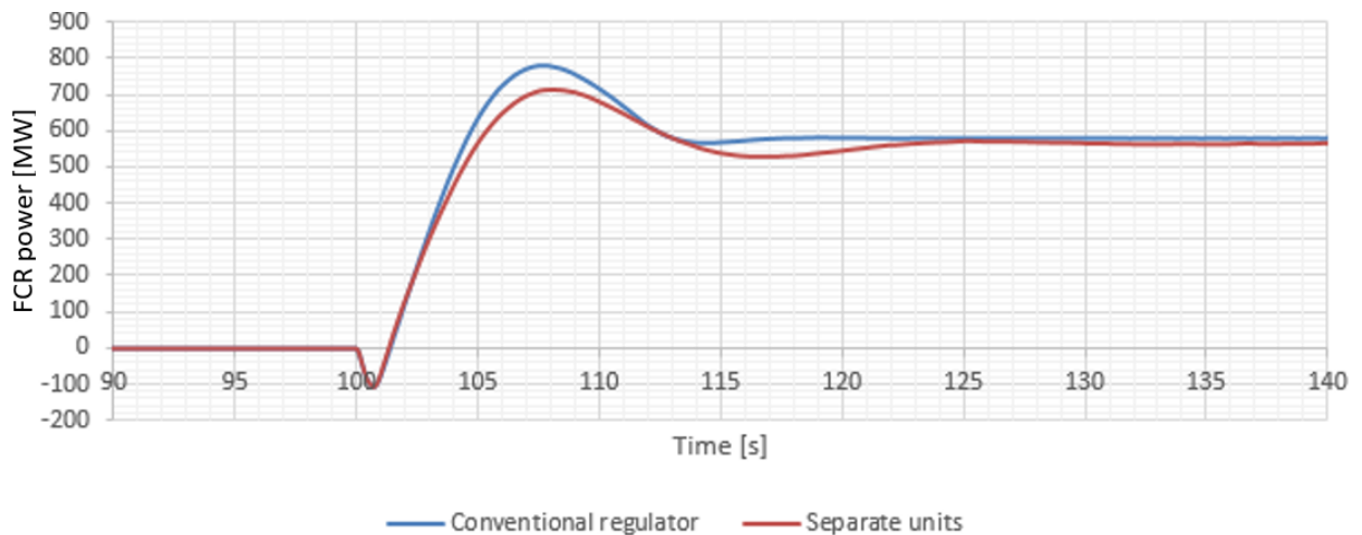
FIGURE 48 FCR POWER RESPONSE AFTER A 600 MW POWER STEP IN A SYSTEM WITH SEPARATE UNITS SUPPLYING FCR-N AND -D (ORANGE), AND A CONVENTIONAL REGULATOR SUPPLYING BOTH FCR-N AND -D (BLUE). PARAMETERS FROM TABLE 6, TABLE 7 AND TABLE 8, BUT WITH K_{i,FCR-D} = 0.2 AND K_{i,FCR-N} = 4 .
