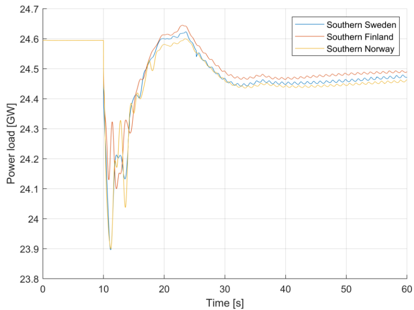
FIGURE 76: ACTIVE POWER LOAD FOR CASE 1 WHEN THE DISTURBANCE OCCUR AT DIFFERENT LOCATIONS, PARAMETER SET 1, FREQUENCY DEPENDENCY: ON, VOLTAGE DEPENDENCY: ON, PSS: ON.
