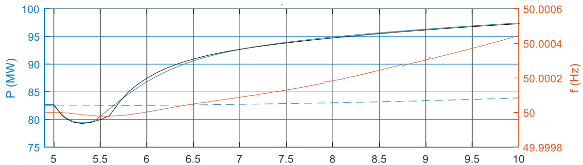
FIGURE 61: COMPARISON OF ONE UNIT'S RESPONSE TO -0.5 Hz STEP IN FREQUENCY REFERENCE IN PSS/E AND IN THE SIMPLIFIED MODEL.
