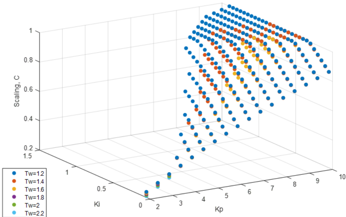
FIGURE 4: 3D-PLOT OF CAPACITY PLOTTED AS A FUNCTION OF PROPORTIONAL GAIN, K_p , AND INTEGRAL GAIN, K_i , FOR DIFFERENT WATER TIME CONSTANTS, T_w (SEE LEGEND). EKS=90 GWS, EKP=300 GWS, BACKLASH=0.5% AND DROOP AT 4%.
