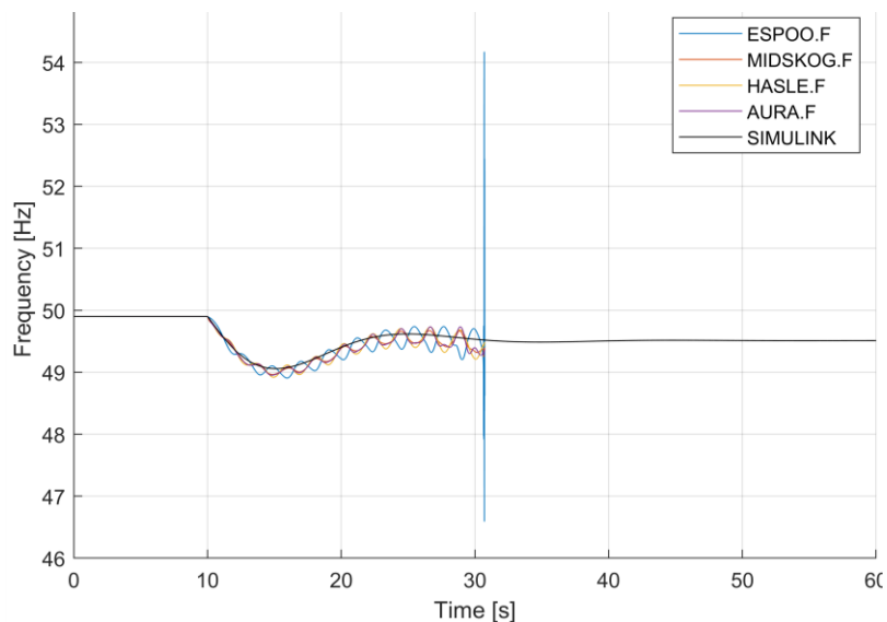
FIGURE 68: FREQUENCY RESPONSE COMPARISON FOR CASE 1, PARAMETER SET 1, DISTURBANCE: SOUTHERN SWEDEN, DEPENDENCY: ON, VOLTAGE DEPENDENCY: OFF, PSS: OFF .
