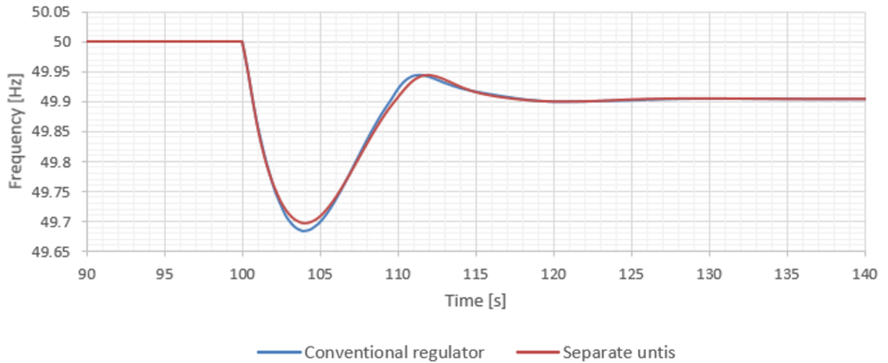
FIGURE 51 FREQUENCY RESPONSE AFTER A 600 MW POWER STEP IN A SYSTEM WITH SEPARATE UNITS SUPPLYING FCR-N AND -D (ORANGE), AND A CONVENTIONAL REGULATOR SUPPLYING BOTH FCR-N AND -D (BLUE). PARAMETERS FROM TABLE 6, TABLE 7 AND TABLE 8, BUT WITH K_{D,FCR-N} = 8 AND K_{D,FCR-D} = 0 .
