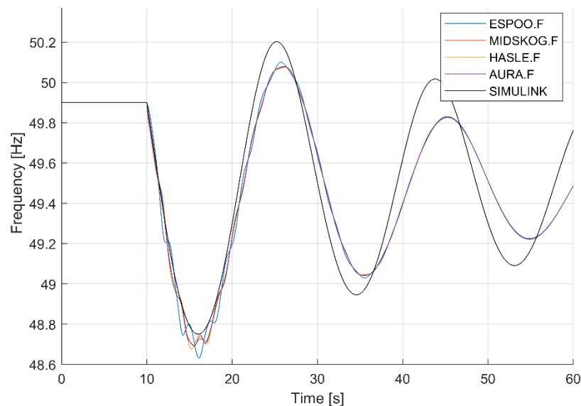
FIGURE 74: FREQUENCY RESPONSE COMPARISON FOR CASE 1, PARAMETER SET 2, DISTURBANCE: SOUTHERN SWEDEN, FREQUENCY DEPENDENCY: ON, VOLTAGE DEPENDENCY: OFF, PSS: ON.
