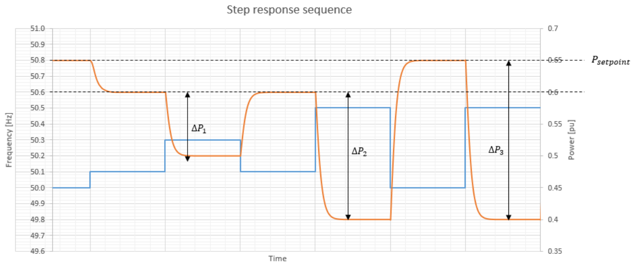
FIGURE 56 EXAMPLE OF STEP RESPONSE FOR FCR-D DOWNWARDS REGULATION FOR DELIVERING BOTH FCR-N AND FCR-D
