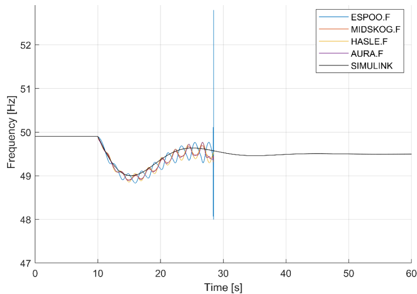
FIGURE 72: FREQUENCY RESPONSE COMPARISON FOR CASE 1, PARAMETER SET 1, DISTURBANCE: SOUTHERN SWEDEN, FREQUENCY DEPENDENCY: OFF, VOLTAGE DEPENDENCY: OFF, PSS: OFF.
