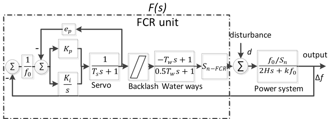
FIGURE 21: NON-LINEAR AGGREGATED REFERENCE MODEL
