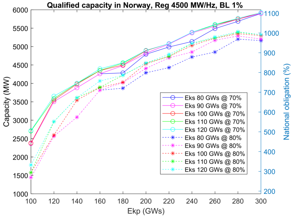
FIGURE 8. ESTIMATED CAPACITY IN NORWAY BASED ON INSTALLED CAPACITY AND DISTRIBUTION OF WATER TIME CONSTANTS. LEFT Y-AXIS IS IN MW AND TO THE RIGHT IN PERCENTAGE OF NATIONAL OBLIGATION (537 MW [FCR MARKET LIQUIDITY NEEDS]). BACKLASH IS SET TO 1 % OF RATED MACHINE POWER. EVALUATED FOR LOADING OF 70 % AND 80 %.
