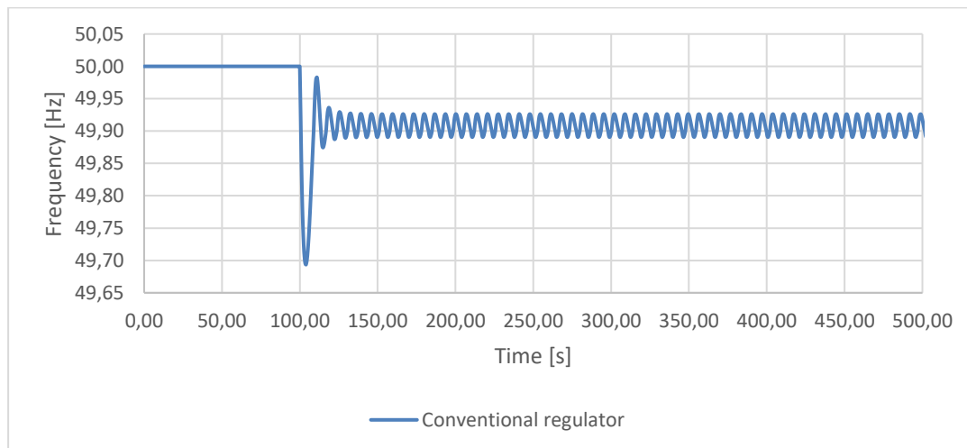
FIGURE 37 FREQUENCY RESPONSE OF A SYSTEM WITH A CONVENTIONAL REGULATOR SWITCHING BETWEEN e_{p,FCR-N} = 0.08 AND e_{p,FCR-D} = 0.04 . THE IMPOSED POWER IMBALANCE IS 600 MW.
