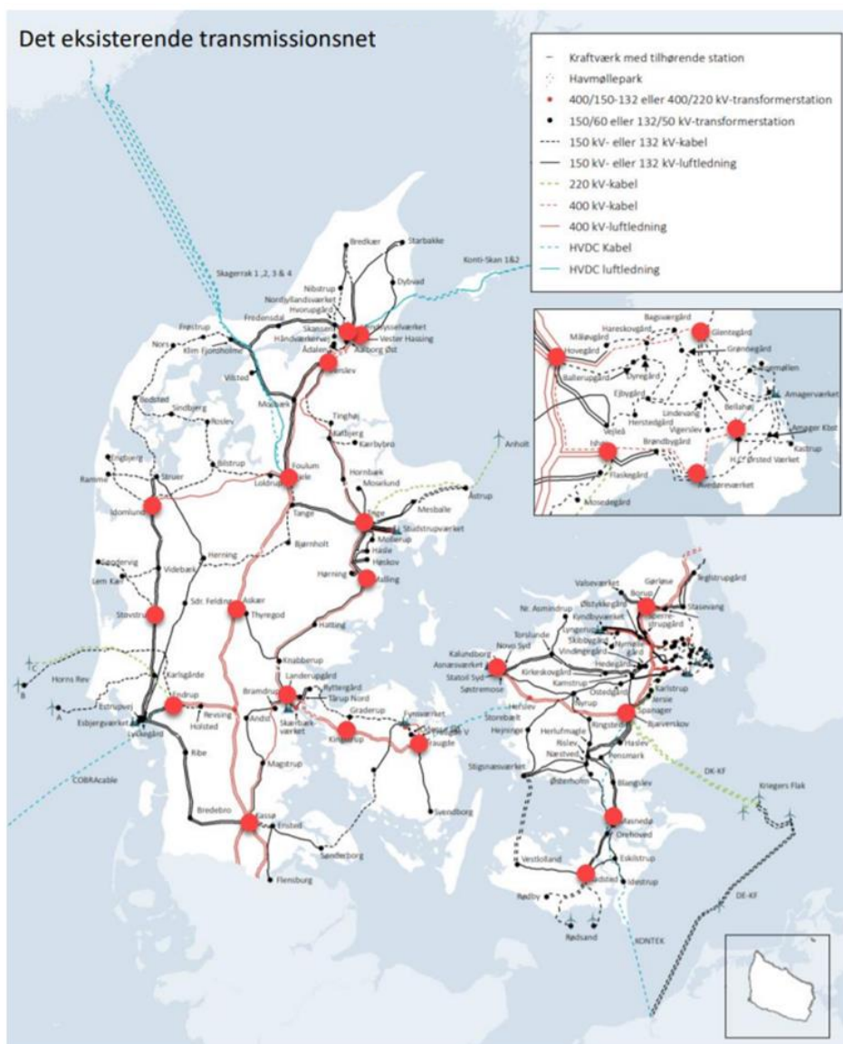
Figur 7: Centrale transmissionsstationer
